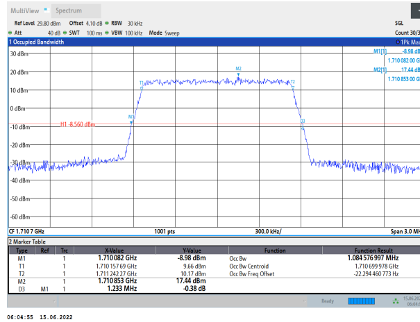
Band66-1.4MHz-QPSK-132322-6RB#0
