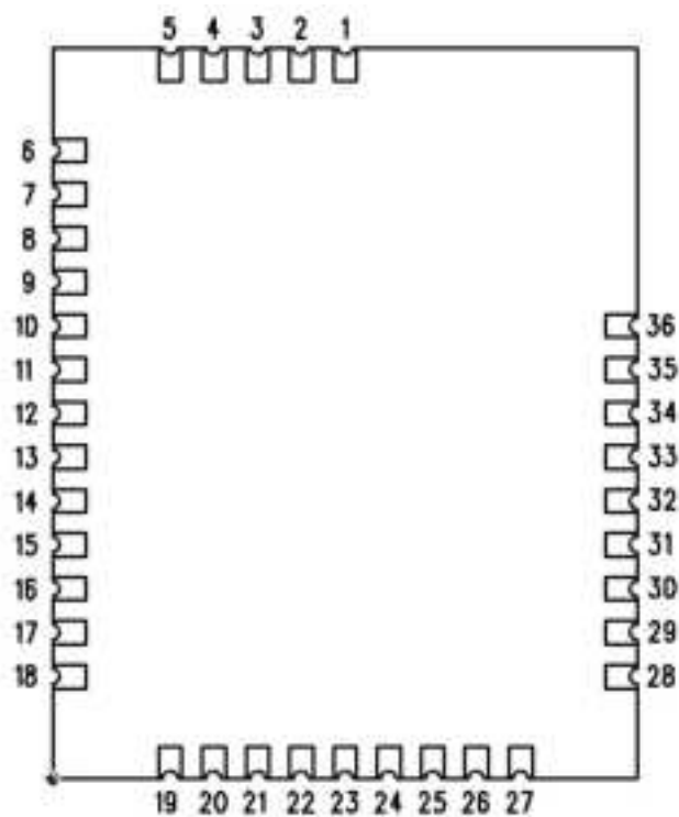
FIG 4 Pin assignment diagram (TOP View)
