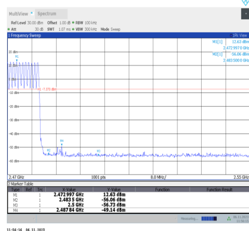
DH5-Ant2-Hop_2480-PASS
