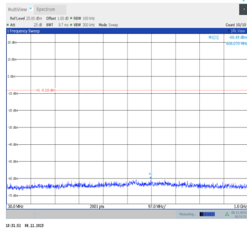
3DH5-Ant2-2480-30~1000-PASS
