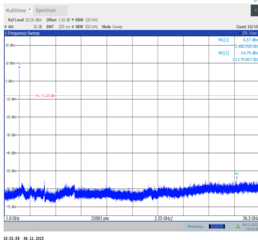
3DH5-Ant2-2480-1000~26500-PASS
