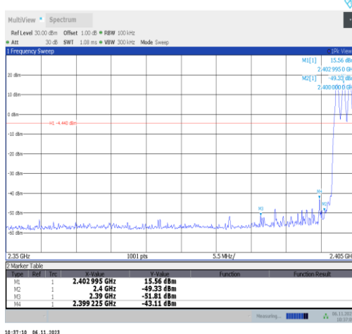
DH5-Ant2-Hop_2402-PASS
