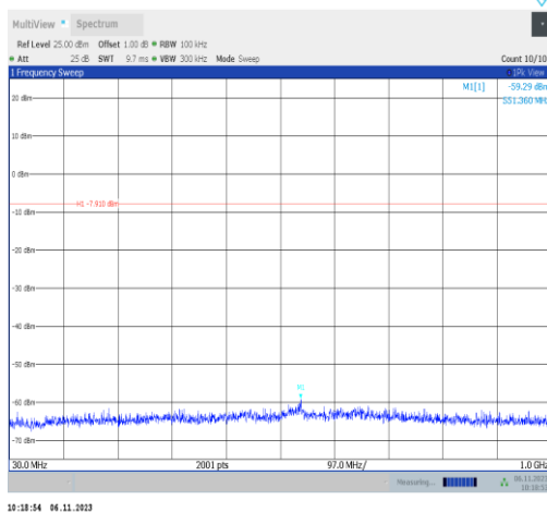
2DH5-Ant2-2480-30~1000-PASS
