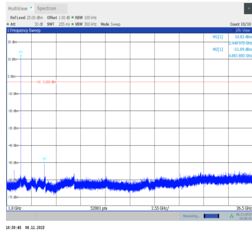
3DH5-Ant2-2441-1000~26500-PASS
