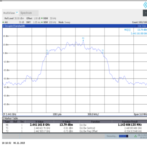
2DH5-Ant2-2441
