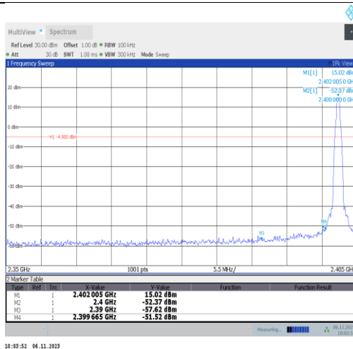
DH5-Ant2-2402-PASS
