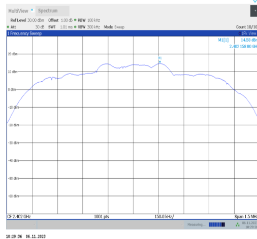
3DH5-Ant2-2402-0~Reference-PASS
