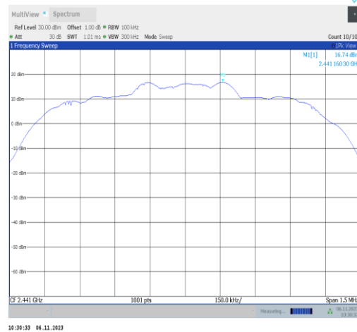
3DH5-Ant2-2441-0~Reference-PASS
