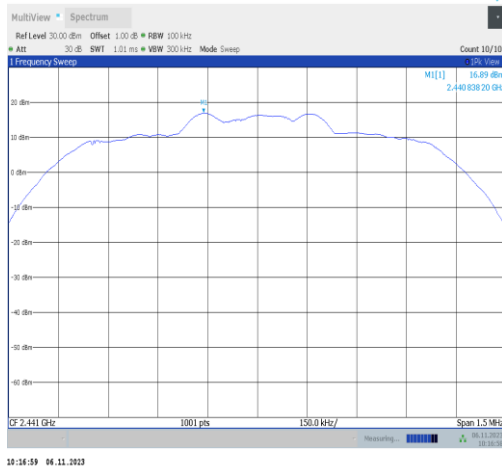
2DH5-Ant2-2441-0~Reference-PASS
