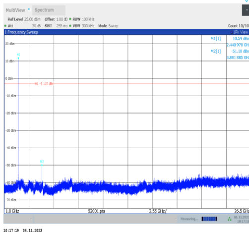
2DH5-Ant2-2441-1000~26500-PASS
