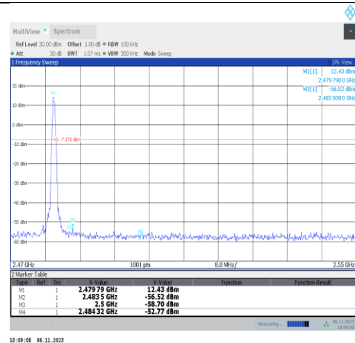
DH5-Ant2-2480-PASS
