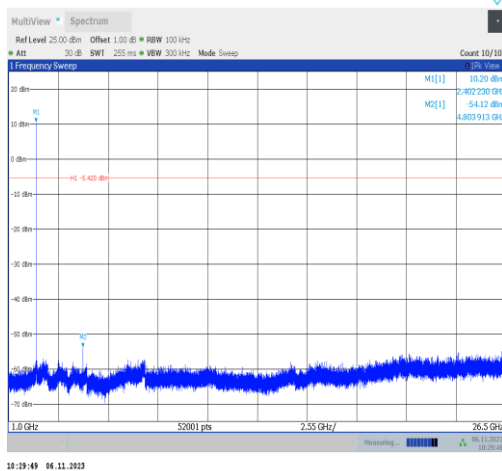
3DH5-Ant2-2402-1000~26500-PASS
