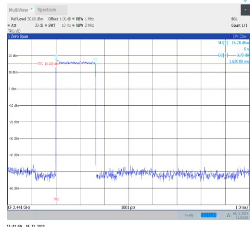
3DH3-Ant2-Hop-PASS
