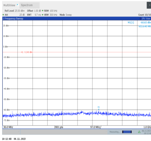
2DH5-Ant2-2402-30~1000-PASS
