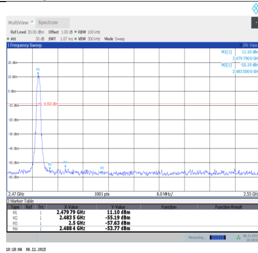
2DH5-Ant2-2480-PASS
