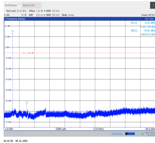
2DH5-Ant2-2402-1000~26500-PASS
