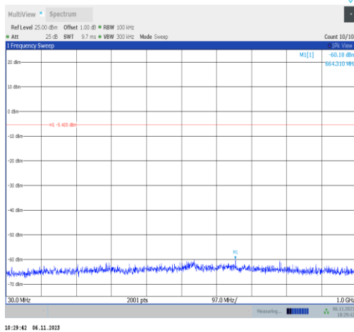
3DH5-Ant2-2402-30~1000-PASS
