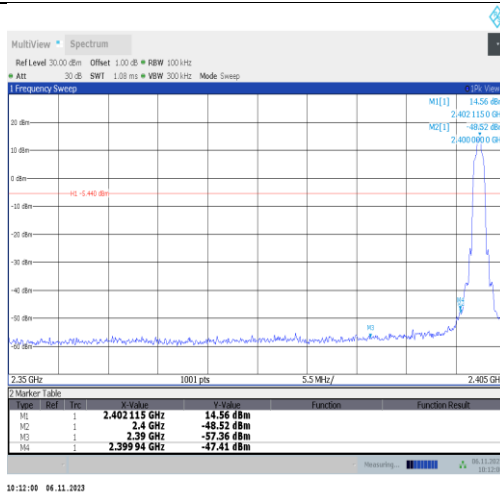
2DH5-Ant2-2402-PASS
