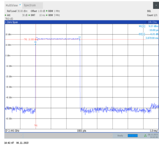
2DH5-Ant2-Hop-PASS
