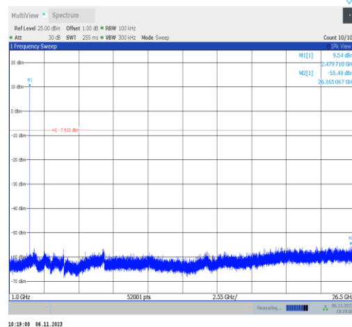
2DH5-Ant2-2480-1000~26500-PASS
