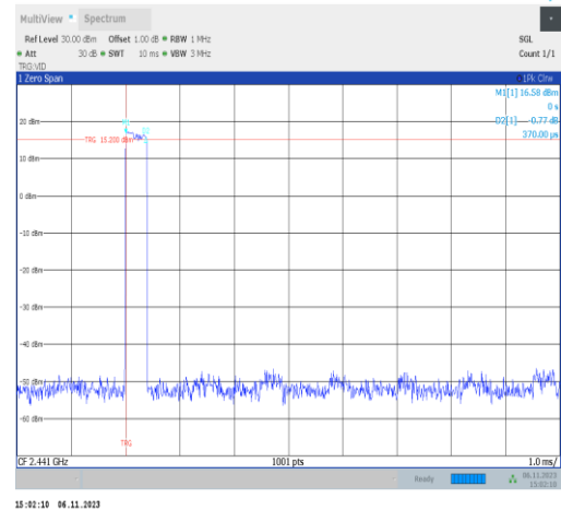
3DH1-Ant2-Hop-PASS
