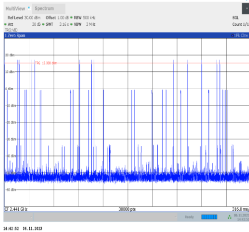
2DH5-Ant2-Hop-PASS
