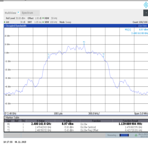
2DH5-Ant2-2480
