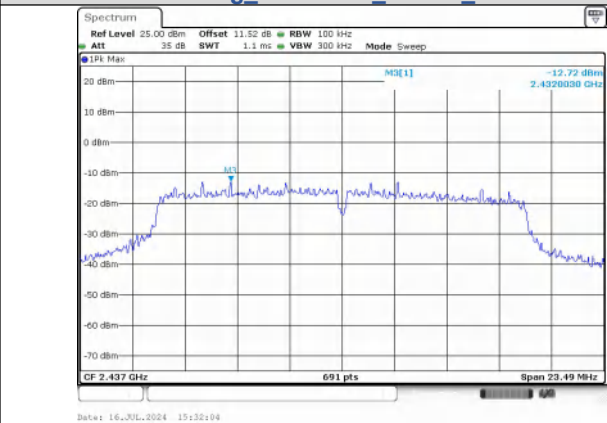
In-Band Reference Level IEEE 802.11g_Channel 6_20MHz_Antenna 0
