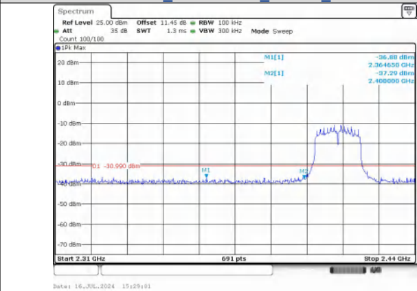
Out Of Band Emission IEEE 802.11g_Channel 1_20MHz_Antenna 0
