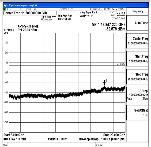
Band4_3MHz_16QAM_19965_1RB#0_3000~20000_3000 0~20000
