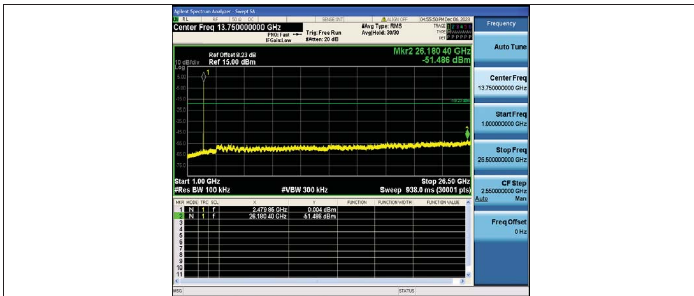
DH5_Ant2_2480_0~Reference
