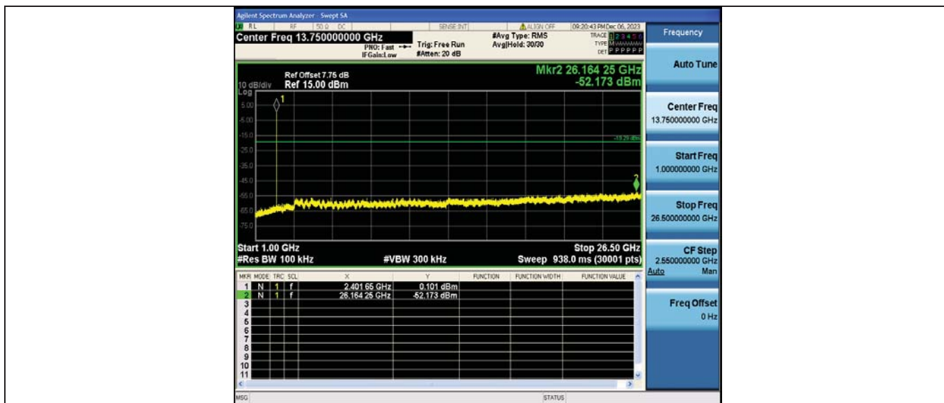
DH5_Ant1_2441_0~Reference
