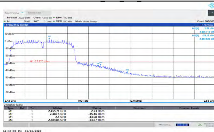
11N40SISO_Ant1_High_2452
