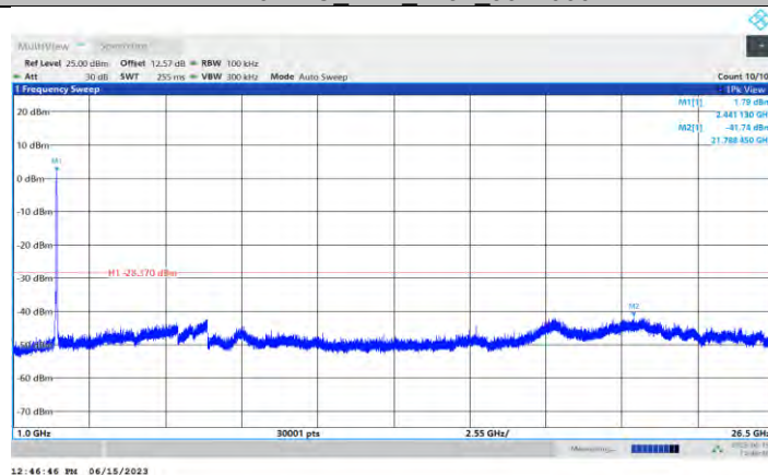
11N40SISO_Ant1_2437_1000~26500
