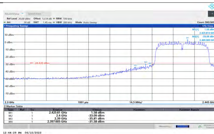
11N40SISO_Ant1_Low_2422
