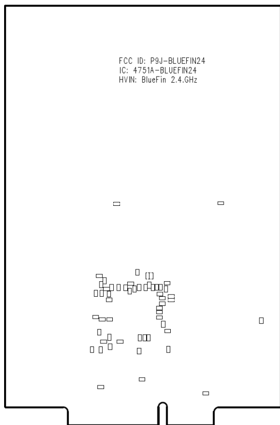
Figure 1. Bottom Side of Silk Screen
