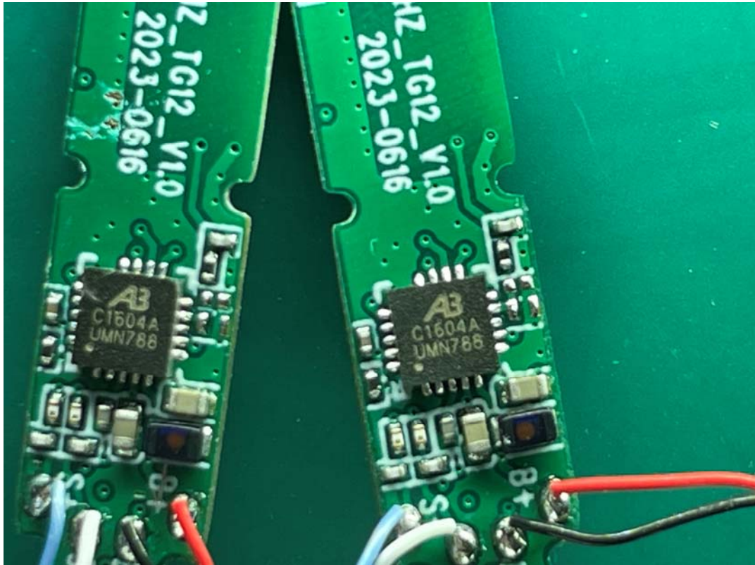
BT Chip
