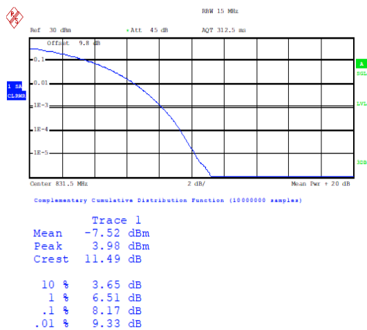
Band26(824-849)-15MHz-QPSK-26865-1RB#0-P ASS
