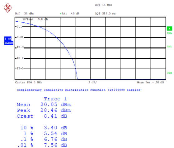
Band26(824-849)-15MHz-QPSK-26915-75RB#0-P ASS
