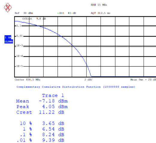
Band26(824-849)-15MHz-QPSK-26915-1RB#0-P ASS
