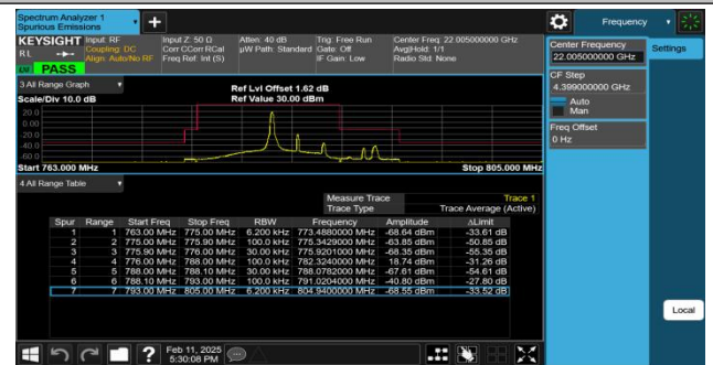
Band13-5MHz-QPSK-23255-1RB#0-PASS
