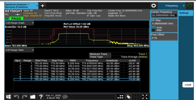
Band13-10MHz-QPSK-23230-50RB#0-PASS
