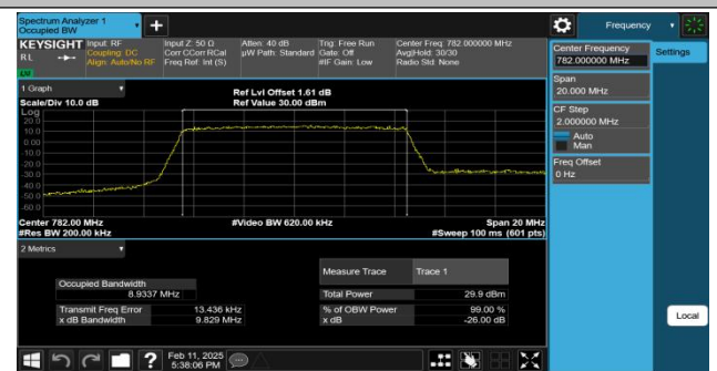
Band13-10MHz-16QAM-23230-50RB#0-PASS
