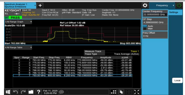
Band13-5MHz-QPSK-23205-25RB#0-PASS
