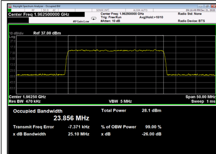
Figure 705: 256QAM 25MHz B.W.; 1962.5MHz, 15kHz - Output
