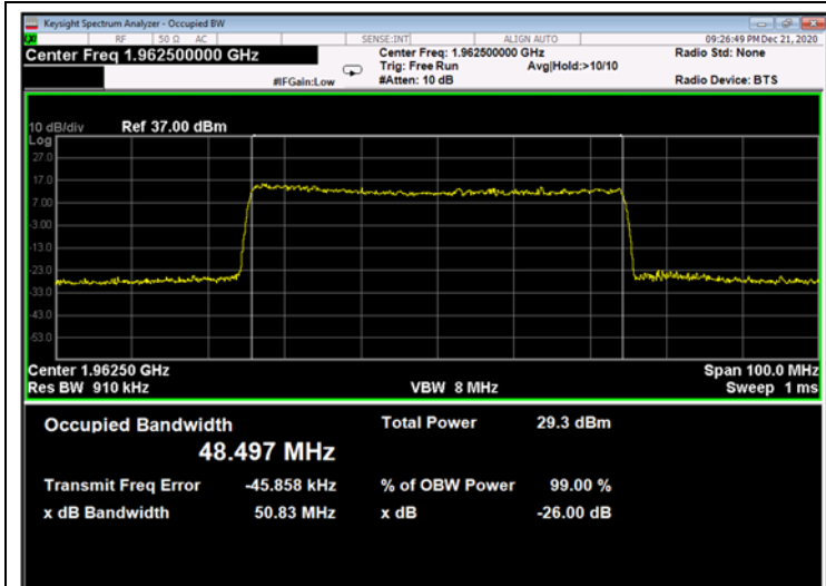
Figure 723: 256QAM 50MHz B.W.; 1962.5MHz, 15kHz - Output
