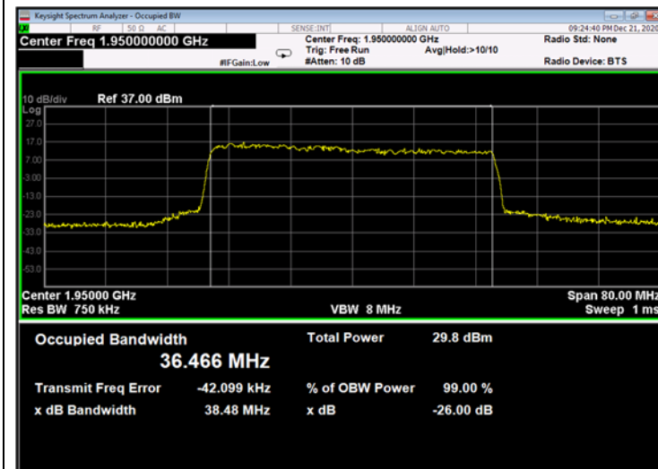
Figure 713: 256QAM 40MHz B.W.; 1950.0MHz, 60kHz - Output
