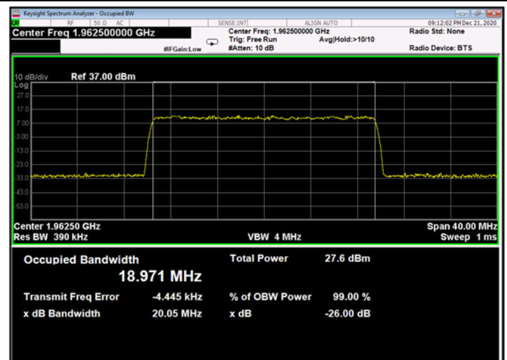
Figure 696: 256QAM 20MHz B.W.; 1962.5MHz, 15kHz - Output
