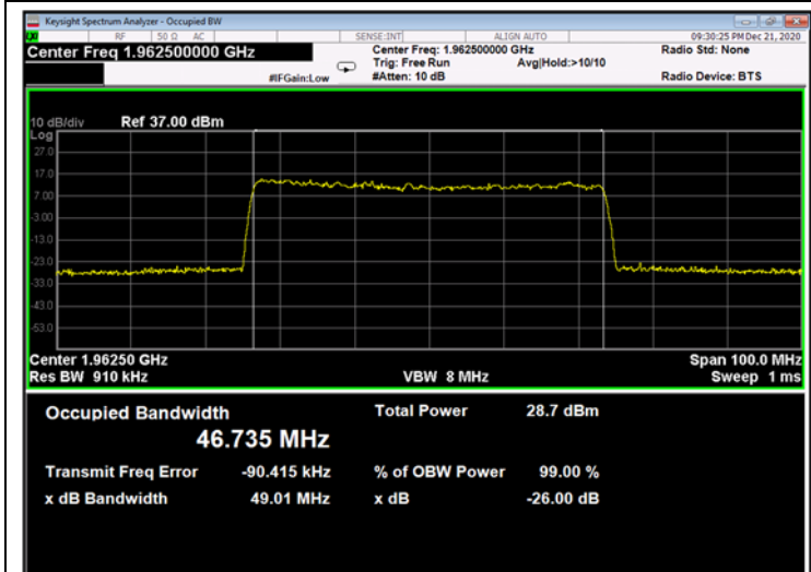
Figure 725: 256QAM 50MHz B.W.; 1962.5MHz, 60kHz - Output
