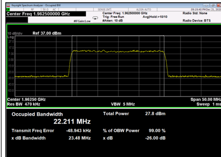
Figure 707: 256QAM 25MHz B.W.; 1962.5MHz, 60kHz - Output
