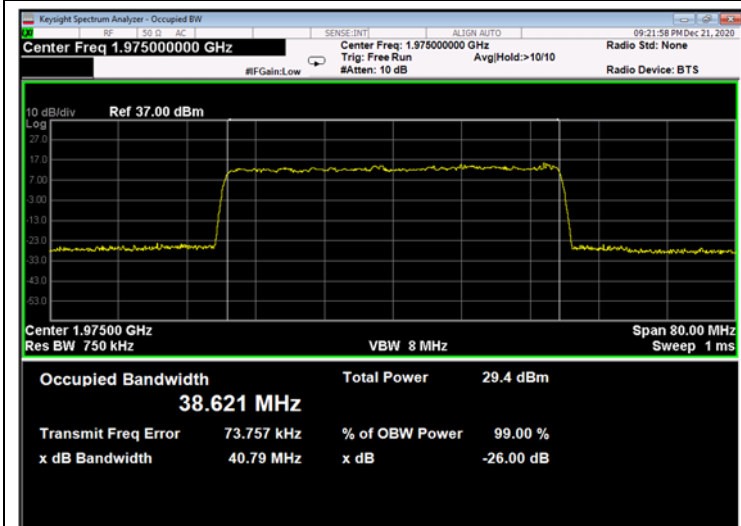
Figure 717: 256QAM 40MHz B.W.; 1975.0MHz, 15kHz - Output
