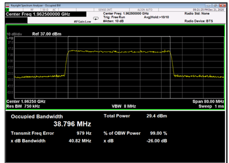
Figure 714: 256QAM 40MHz B.W.; 1962.5MHz, 15kHz - Output
