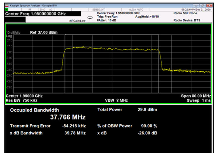
Figure 712: 256QAM 40MHz B.W.; 1950.0MHz, 30kHz - Output
