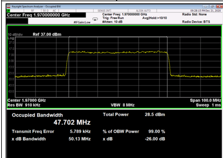
Figure 727: 256QAM 50MHz B.W.; 1970.0MHz, 30kHz - Output
