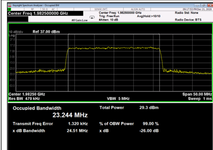
Figure 709: 256QAM 25MHz B.W.; 1982.5MHz, 30kHz - Output
