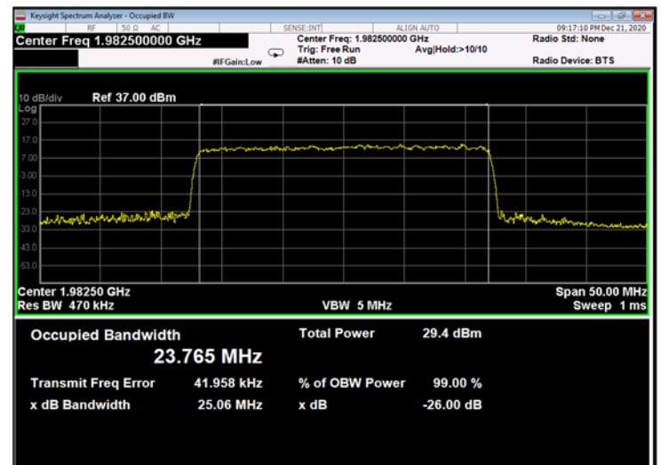
Figure 708: 256QAM 25MHz B.W.; 1982.5MHz, 15kHz - Output
