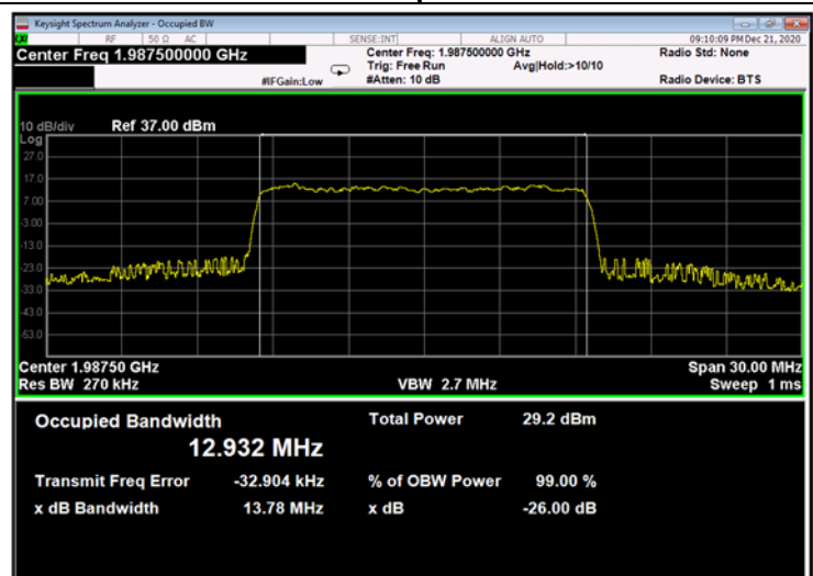
Figure 692: 256QAM 15MHz B.W.; 1987.5MHz, 60kHz - Output
