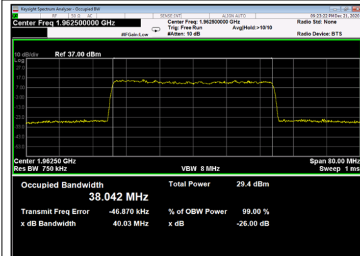
Figure 715: 256QAM 40MHz B.W.; 1962.5MHz, 30kHz - Output
