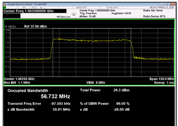
Figure 732: 256QAM 60MHz B.W.; 1962.5MHz, 60kHz - Output
