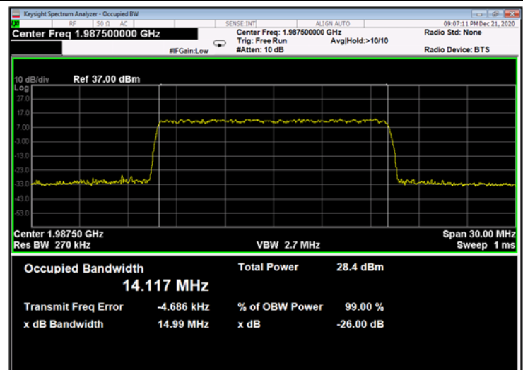
Figure 690: 256QAM 15MHz B.W.; 1987.5MHz, 15kHz - Output
