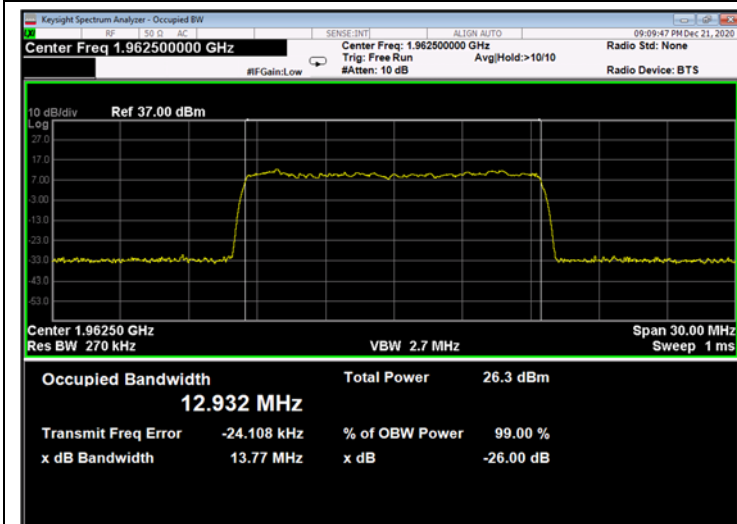
Figure 689: 256QAM 15MHz B.W.; 1962.5MHz, 60kHz - Output
