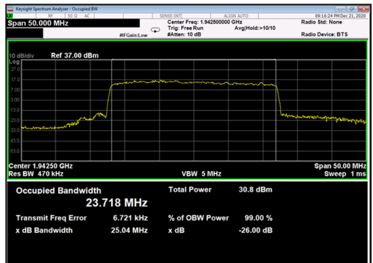
Figure 702: 256QAM 25MHz B.W.; 1942.5MHz, 15kHz - Output
