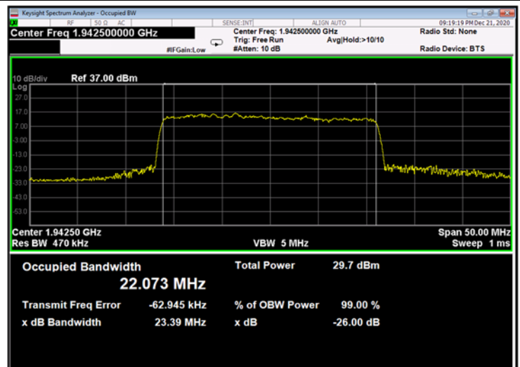
Figure 704: 256QAM 25MHz B.W.; 1942.5MHz, 60kHz - Output
