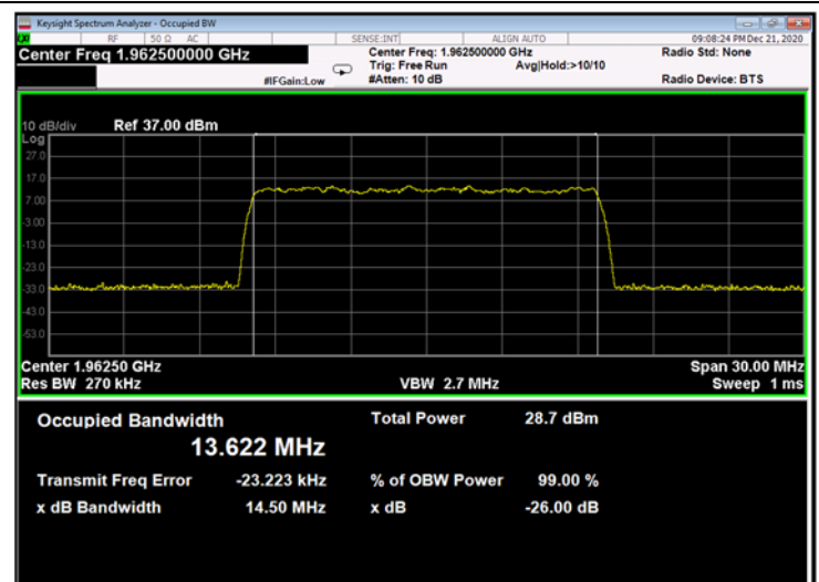
Figure 688: 256QAM 15MHz B.W.; 1962.5MHz, 30kHz - Output
