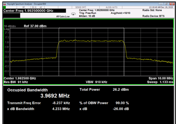
Figure 740: QPSK 5MHzC.S; 1992.5MHz, 30kHz - Output
