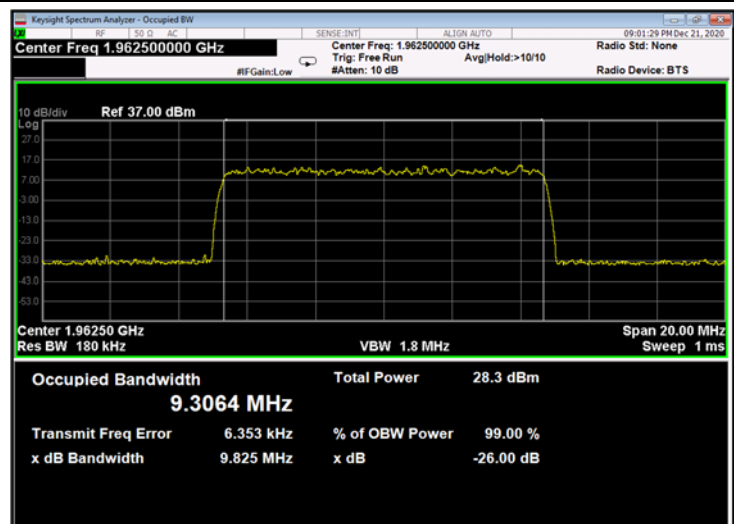
Figure 678: 256QAM 10MHz B.W.; 1962.5MHz, 15kHz - Output
