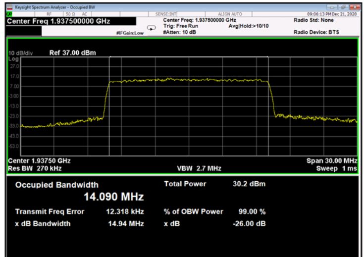
Figure 684: 256QAM 15MHz B.W.; 1937.5MHz, 15kHz - Output
