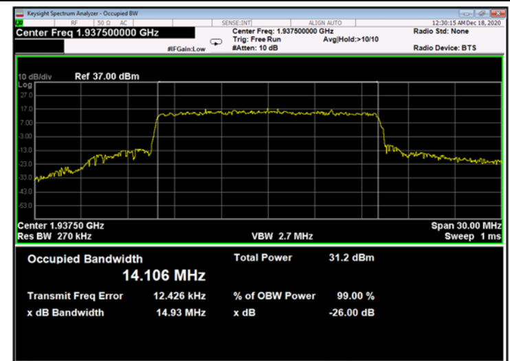
Figure 750: QPSK 15MHz B.W.; 1937.5MHz, 15kHz - Output
