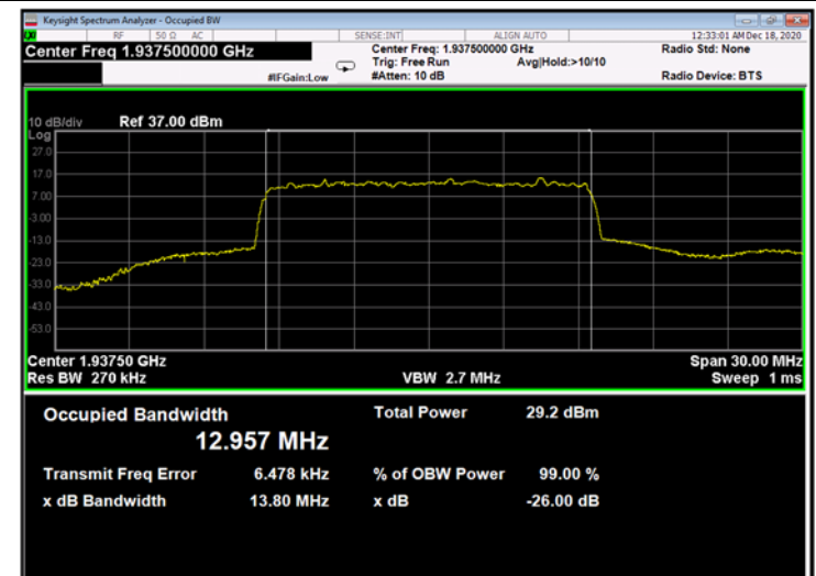
Figure 752: QPSK 15MHz B.W.; 1937.5MHz, 60kHz - Output
