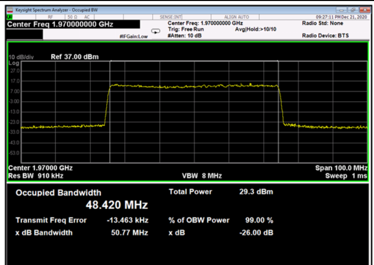
Figure 726: 256QAM 50MHz B.W.; 1970.0MHz, 15kHz - Output
