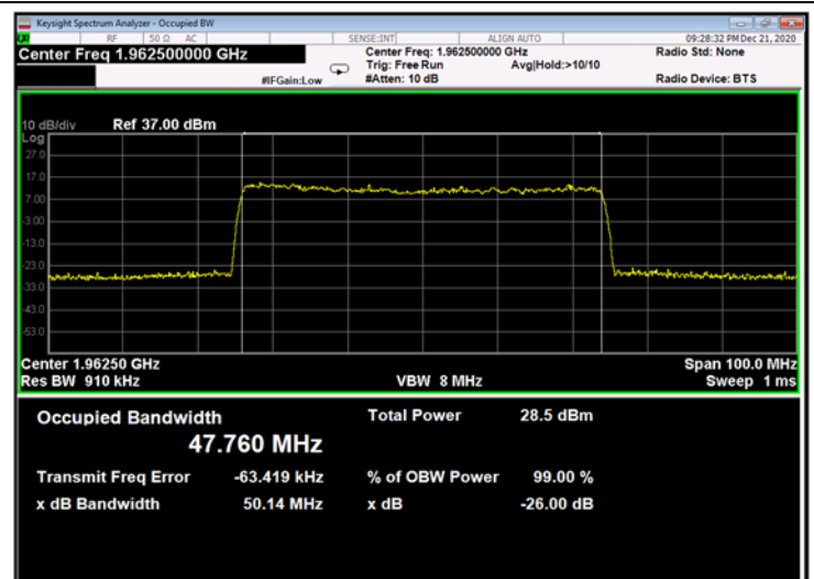
Figure 724: 256QAM 50MHz B.W.; 1962.5MHz, 30kHz - Output
