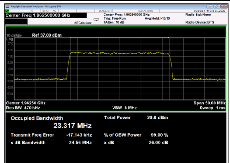
Figure 706: 256QAM 25MHz B.W.; 1962.5MHz, 30kHz - Output
