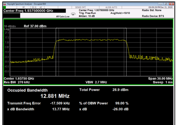
Figure 686: 256QAM 15MHz B.W.; 1937.5MHz, 60kHz - Output
