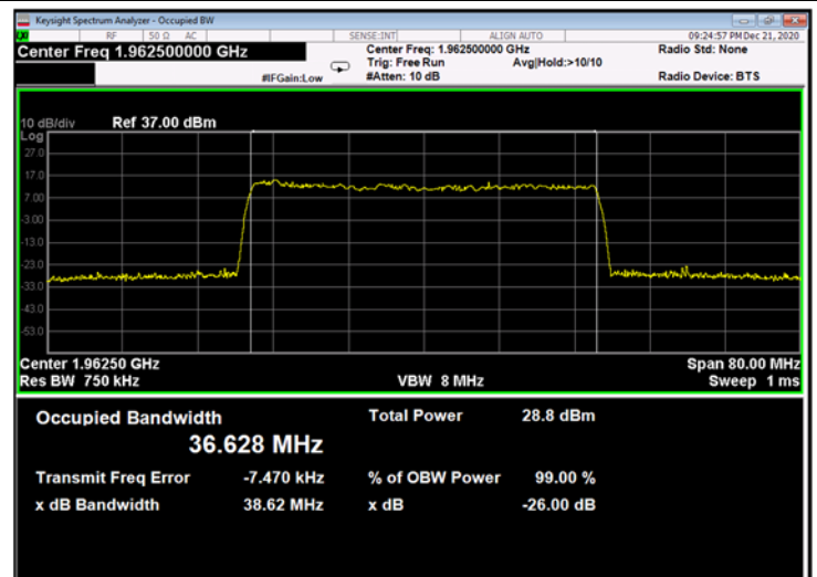
Figure 716: 256QAM 40MHz B.W.; 1962.5MHz, 60kHz - Output
