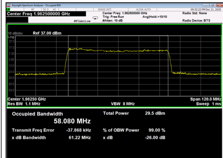
Figure 731: 256QAM 60MHz B.W.; 1962.5MHz, 30Hz - Output
