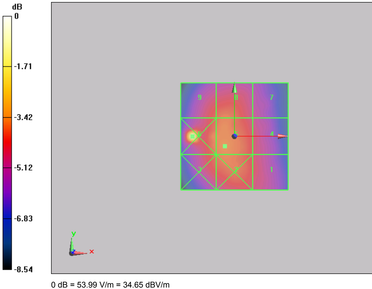
Figure 15 HAC RF E-Field CDMA BC10 Channel 476
