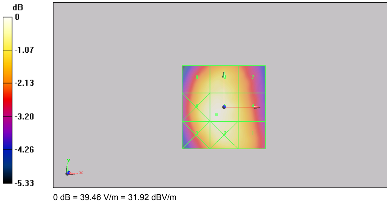
Figure 10 HAC RF E-Field CDMA BC0 Channel 1013
