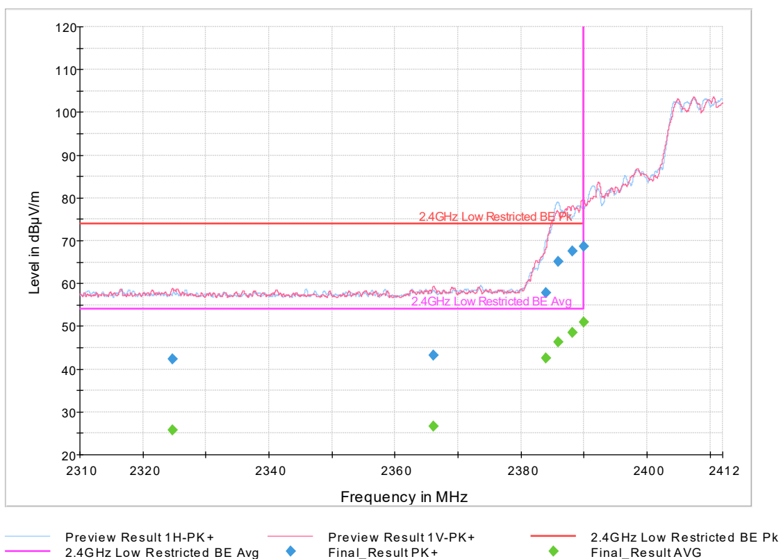
Plot 11. Low Bandedge 802.11n 40 MHz Mode, Low Channel
