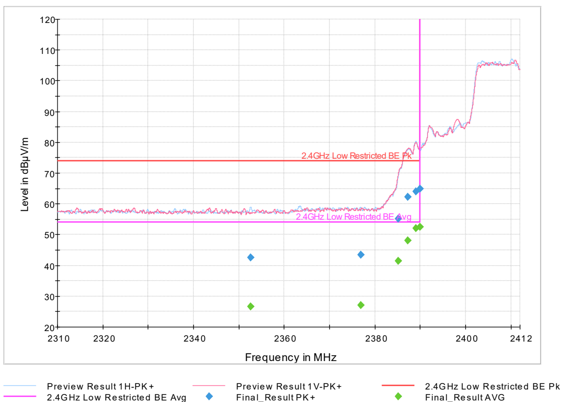
Plot 9. Low Bandedge 802.11ac Mode, Low Channel
