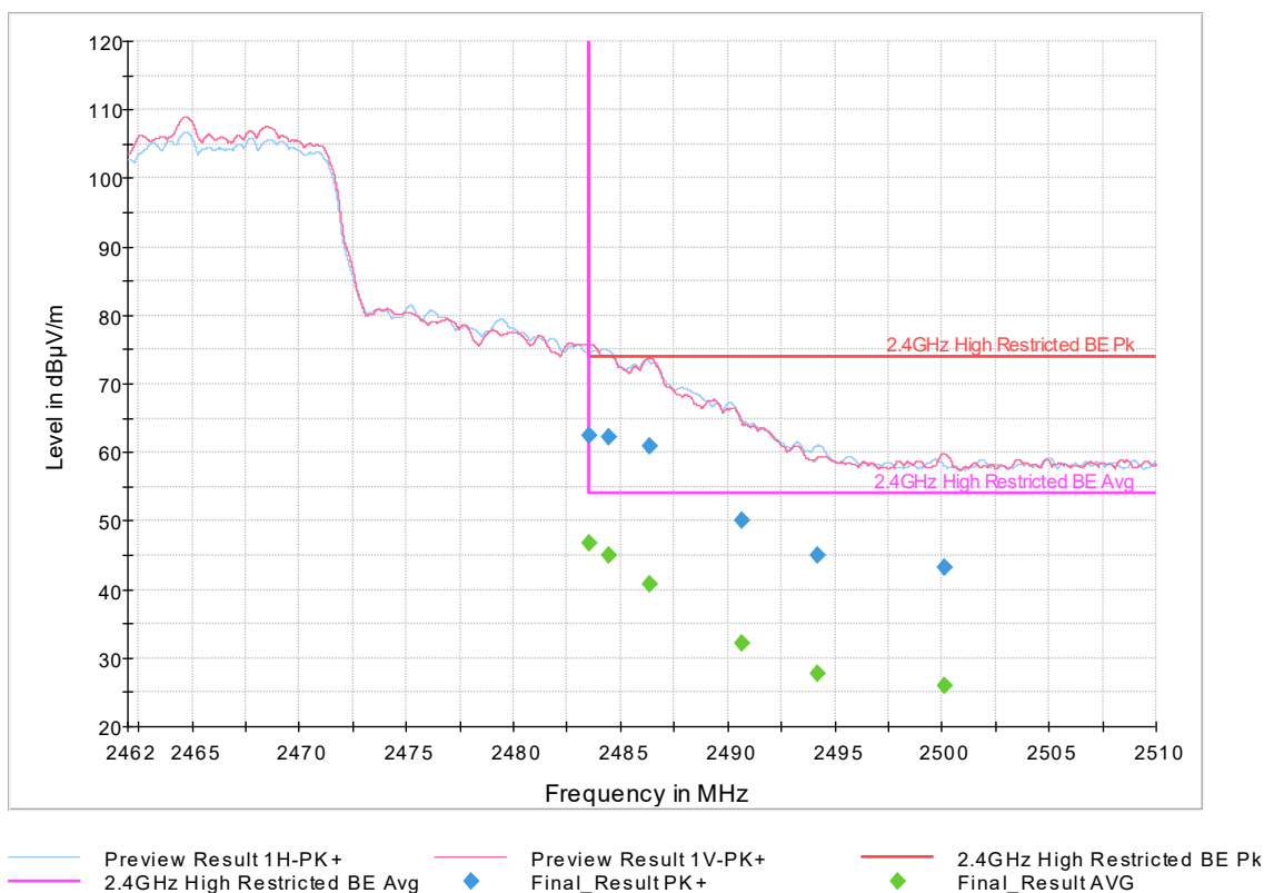
Plot 22. High Bandedge 802.11ax Mode, High Channel
