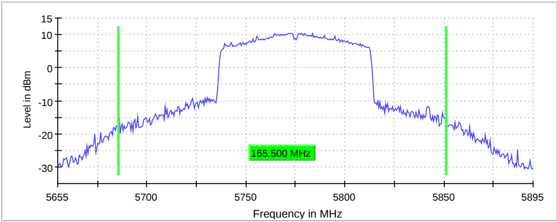
26 dB Bandwidth
