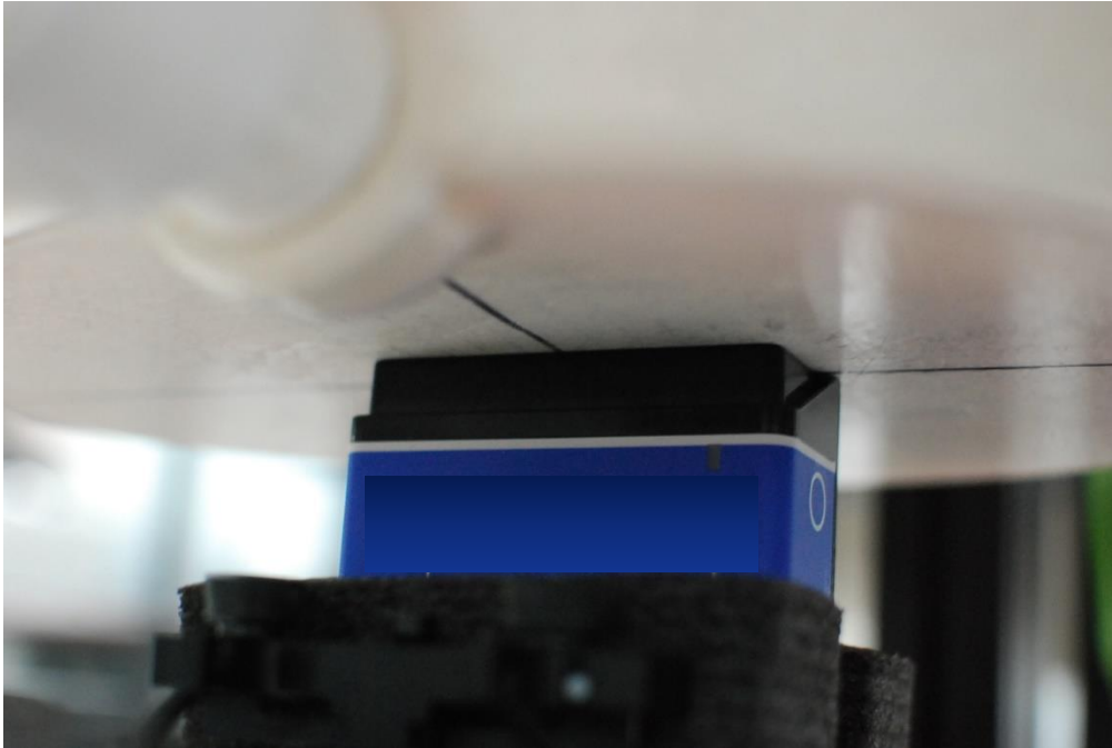
SAR Test Setup Photo 3 – Top Edge at 0mm
