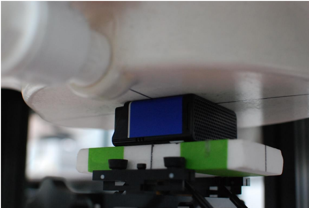
SAR Test Setup Photo 2 – Front Side at 0mm
