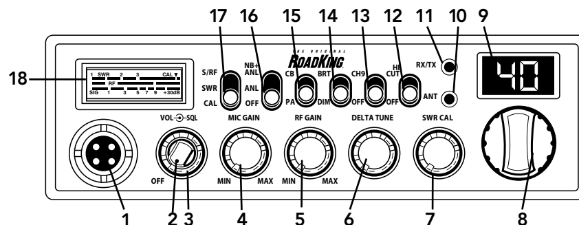
FRONT VIEW - RKCB CLASSIC
