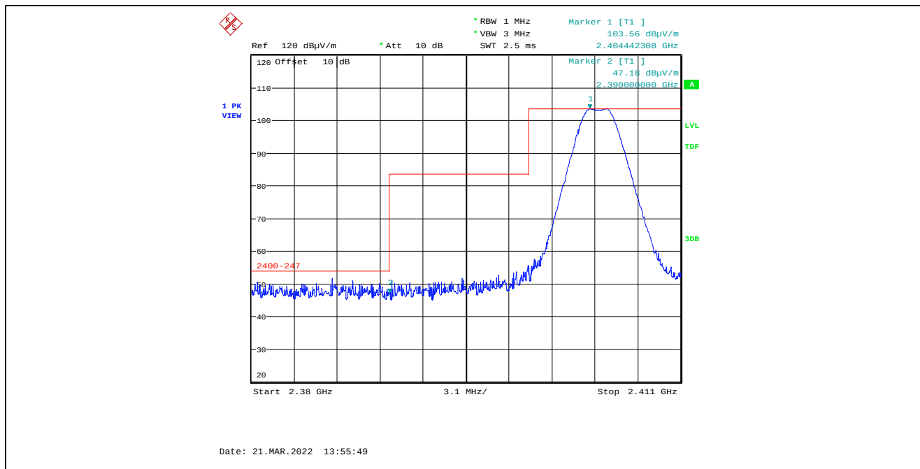
Plot 5.4.4.2.2.1. Band-Edge RF Radiated Emissions at 3 m, Vertical Polarization, Peak Low End of Frequency Band, 2405 MHz, 7 dBm Power Setting
