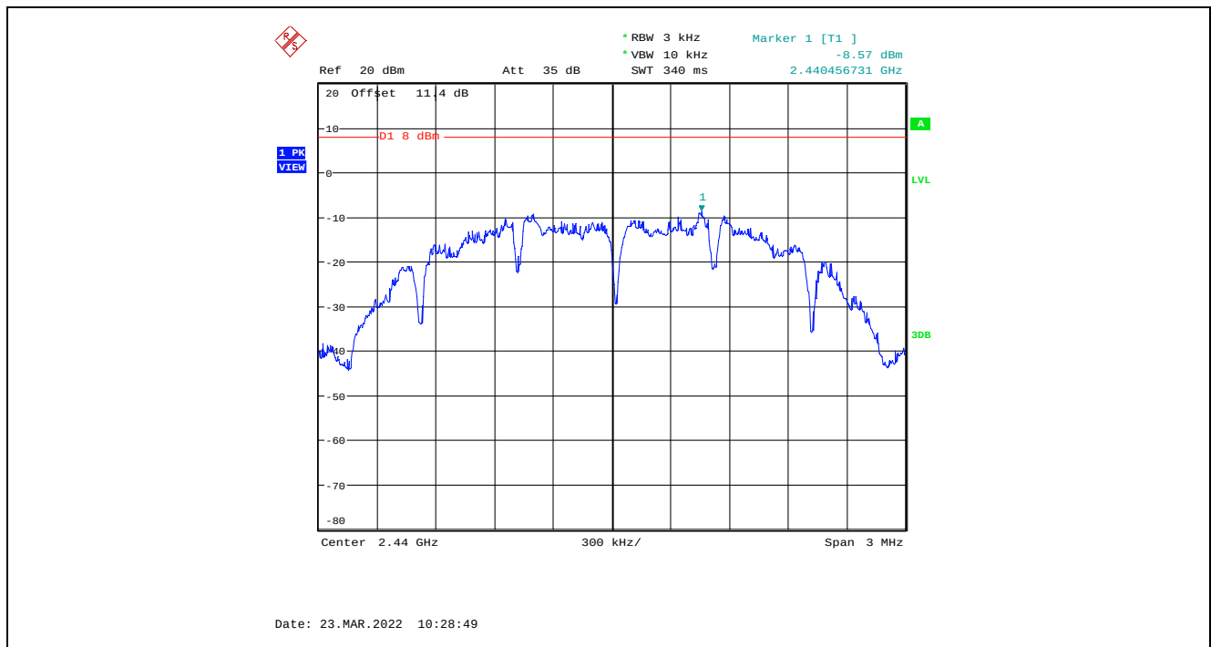
Plot 5.5.4.2. Power Spectral Density, QPSK Modulation, 7 dBm Power Setting, 2440 MHz
