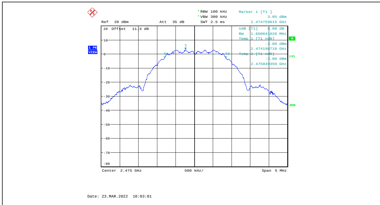
Plot 5.2.4.3. 6 dB Bandwidth, QPSK Modulation, 7 dBm Power Setting, 2475 MHz
