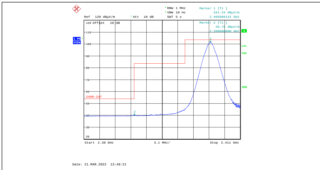
Plot 5.4.4.2.4. Band-Edge RF Radiated Emissions at 3 m, Horizontal Polarization, Average Low End of Frequency Band, 2405 MHz, 7 dBm Power Setting
