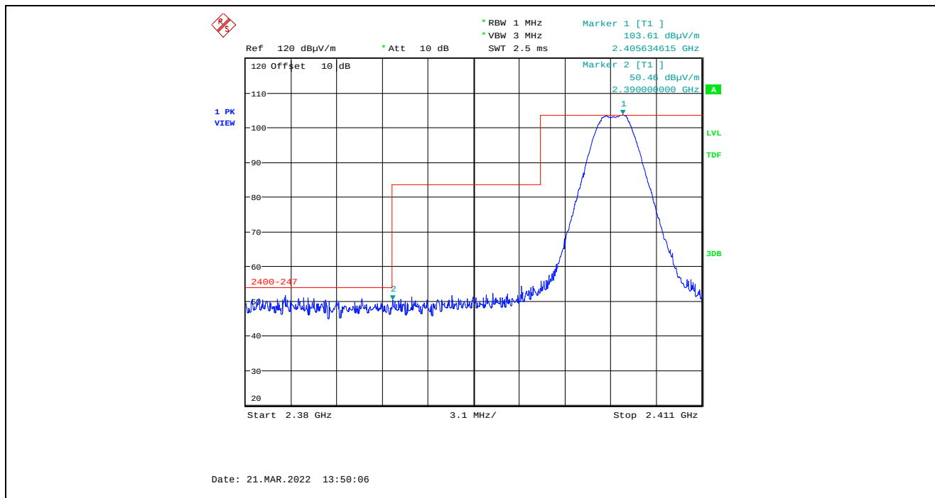
Plot 5.4.4.2.3. Band-Edge RF Radiated Emissions at 3 m, Horizontal Polarization, Peak Low End of Frequency Band, 2405 MHz, 7 dBm Power Setting
