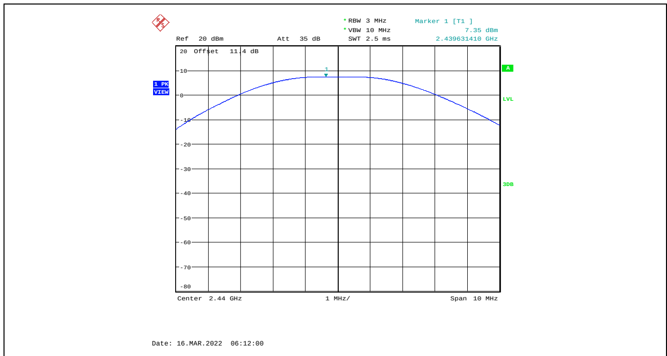
Plot 5.3.4.2. Maximum Peak Conducted Output Power, QPSK Modulation, 7 dBm Power Setting, 2440 MHz
