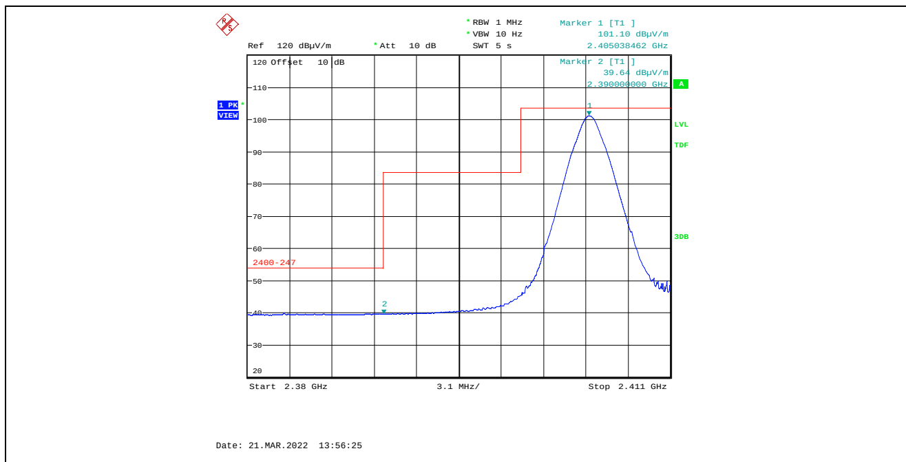
Plot 5.4.4.2.2.2. Band-Edge RF Radiated Emissions at 3 m, Vertical Polarization, Average Low End of Frequency Band, 2405 MHz, 7 dBm Power Setting
