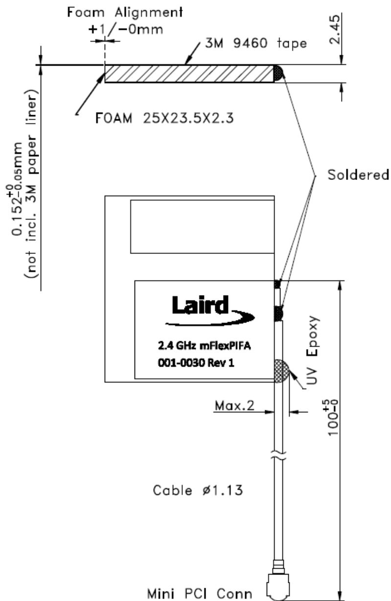
Figure 1: Physical dimensions
