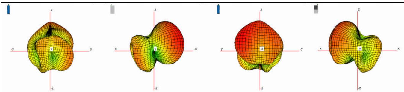
ANT5-WIFI 5800MHz
