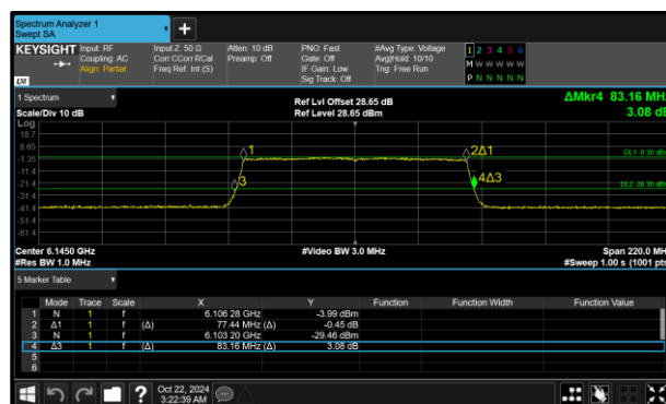
Figure 162 - 802.11ax HE80 SU LPI Maximum 26 dB EBW
