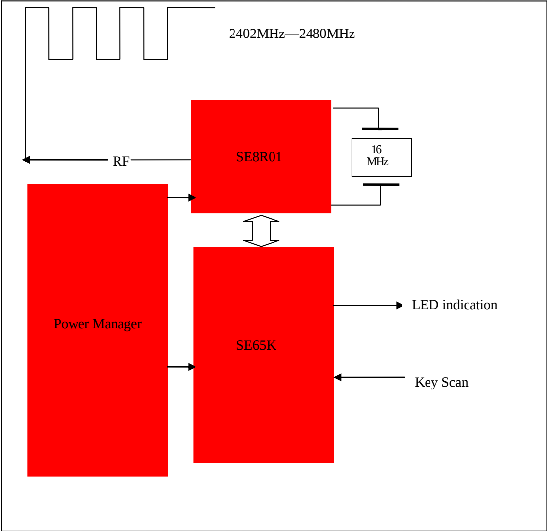
Wireless Keyboard Functional block diagram
