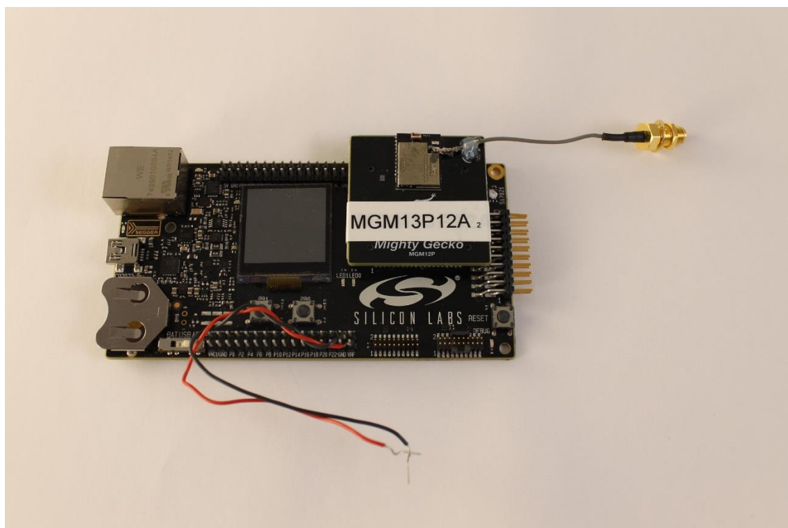
Photograph 2. DUT 2
