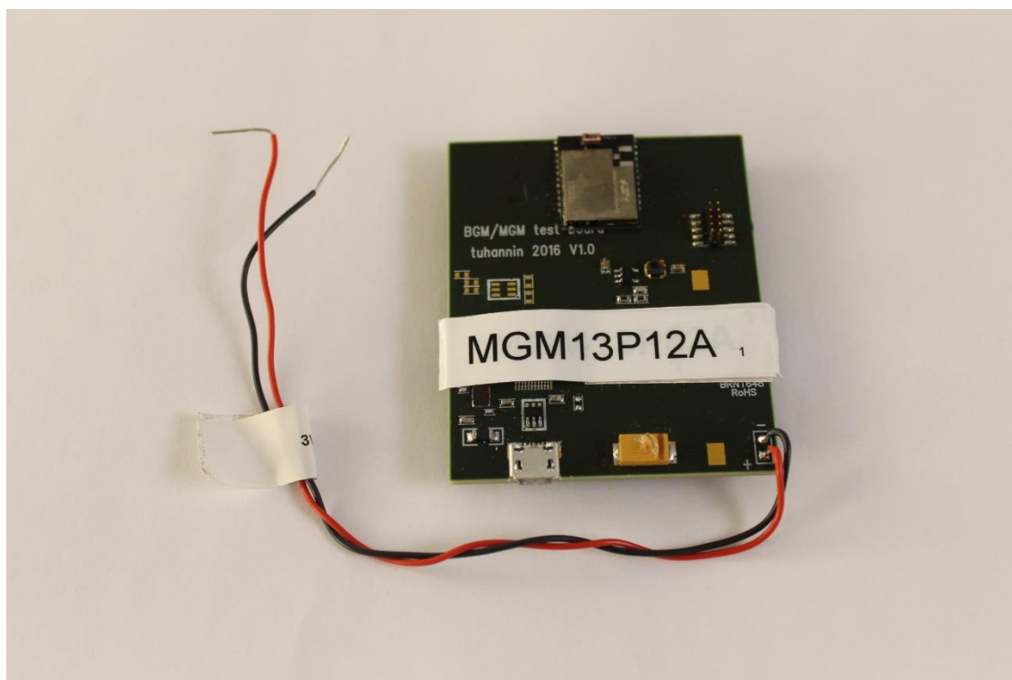
Photograph 1. DUT 1
