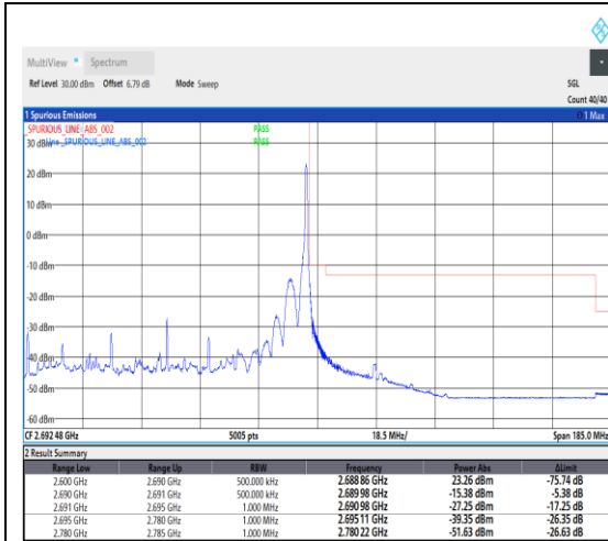
1-N41--30-90-H-2-DFT-PI2BPSK-Edge_1RB _Right-1@244-Ant1-1--PASS-see graph
