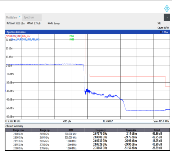
1-N41--30-90-H-3-DFT-PI2BPSK-Outer_Full- 243@0-Ant1-1--PASS-see graph
