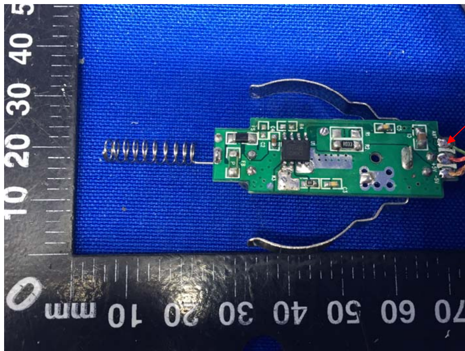
FM Antenna
