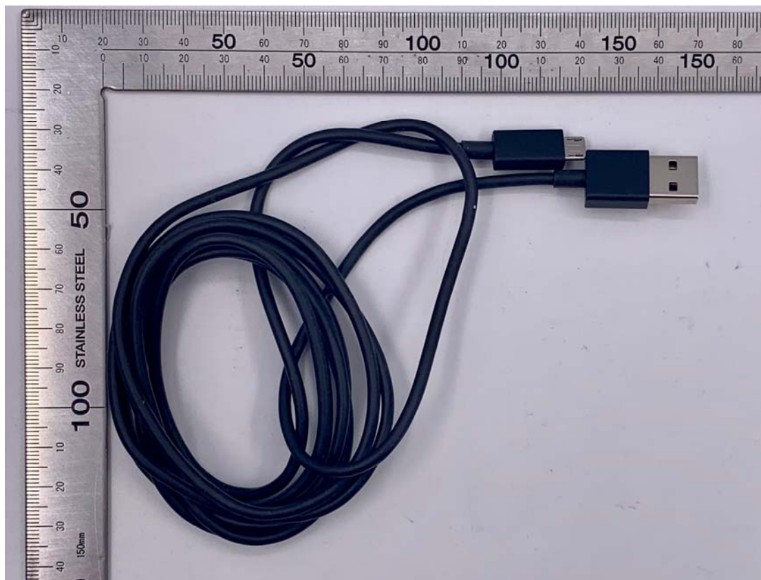
The USB cable View (KLC-3103 by Suzhou KELI TECHNOLOGY DEVELOPMENT CO., LTD.)
