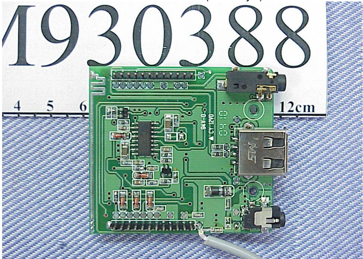
Photos 27 (Multi-Player) Interface Board/Front Side
