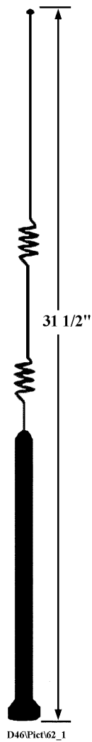
Figure 1: 46-0062-001 Antenna dimensions (For Reference Only)
