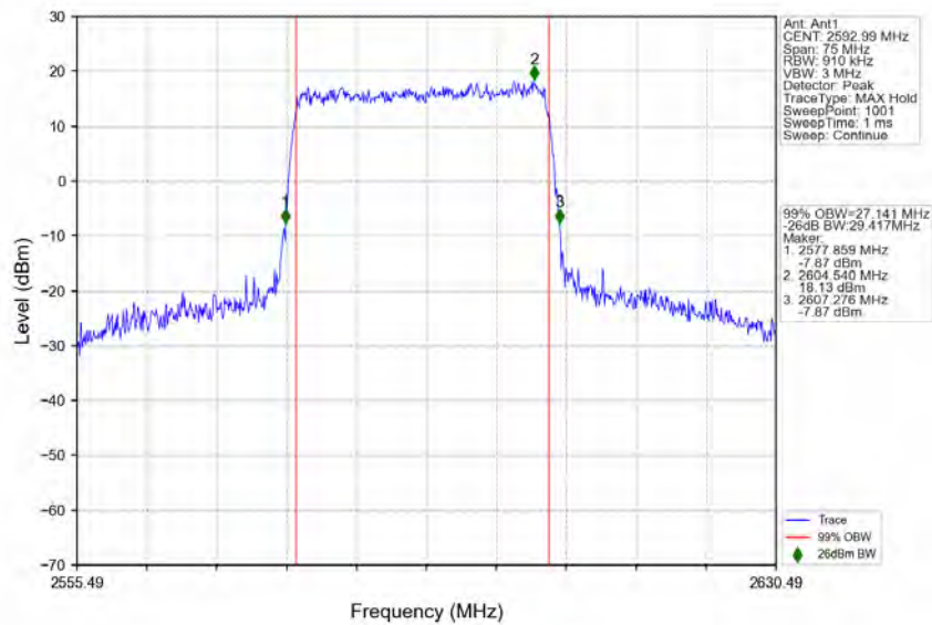
n41_30kHz_SISO_NTNV_30MHz_DFT-s-OFDM_16_QAM_2592.99MHz_Outer_Full
