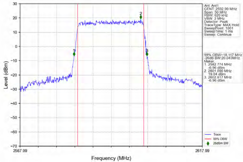
n41_30kHz_SISO_NTNV_20MHz_DFT-s-OFDM PI/2 BPSK_2592.99MHz_Outer_Full
