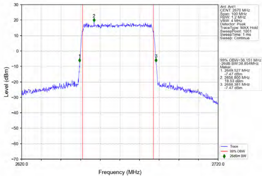
n41_30kHz_SISO_NTNV_40MHz_DFT-s-OFDM_QPSK_2670MHz_Outer_Full
