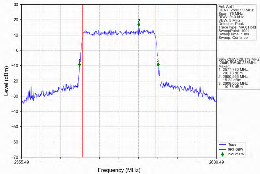
n41_30kHz_SISO_NTNV_30MHz_CP-OFDM_256_QAM_2592.99MHz_Outer_Full
