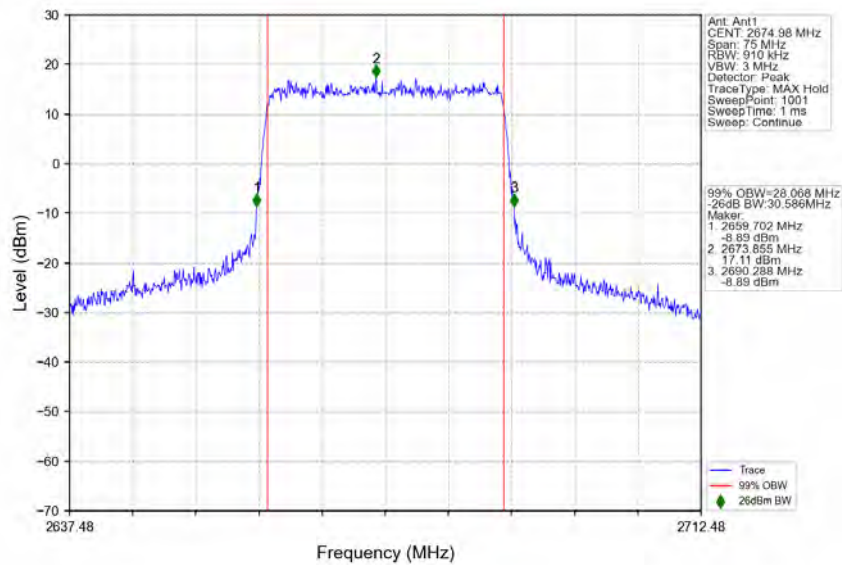
n41_30kHz_SISO_NTNV_30MHz_CP-OFDM_QPSK_2674.98MHz_Outer_Full
