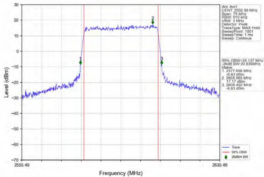
n41_30kHz_SISO_NTNV_30MHz_CP-OFDM_16_QAM_2592.99MHz_Outer_Full
