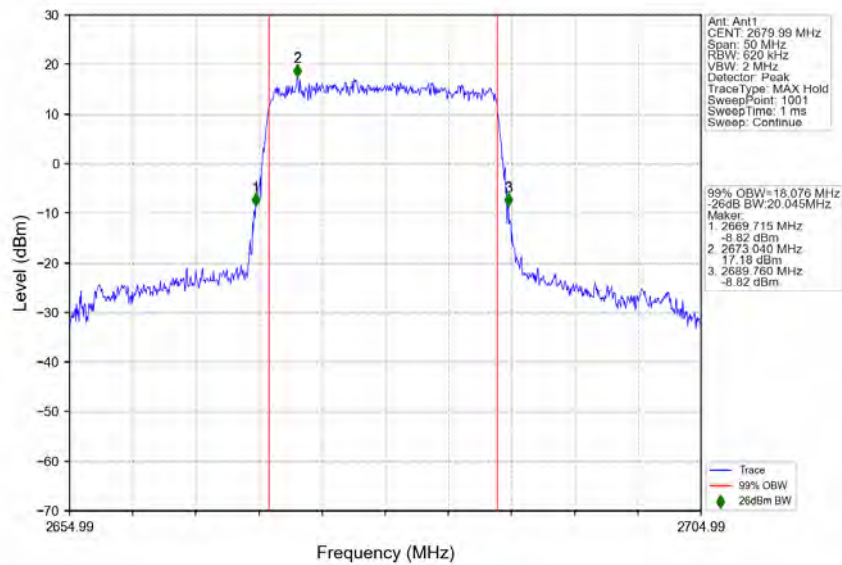
n41_30kHz_SISO_NTNV_20MHz_DFT-s-OFDM_64_QAM_2679.99MHz_Outer_Full
