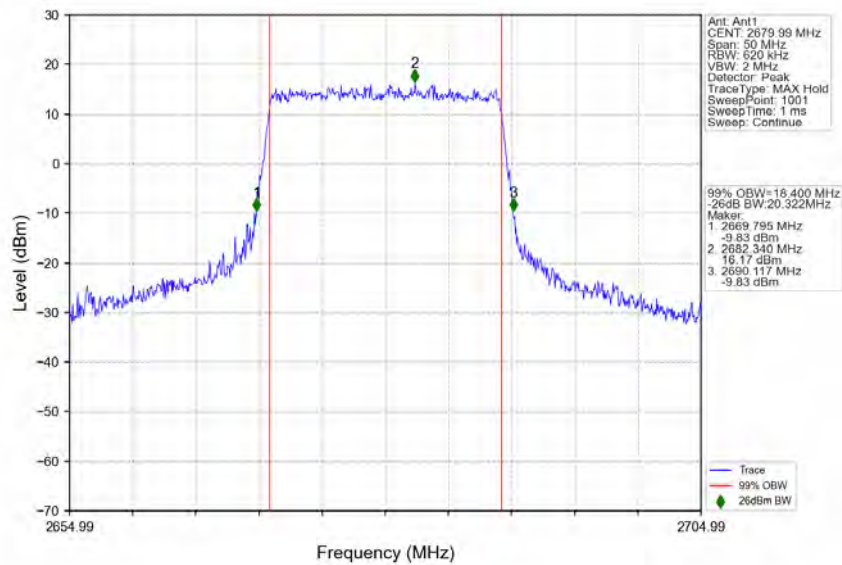
n41_30kHz_SISO_NTNV_20MHz_CP-OFDM_64_QAM_2679.99MHz_Outer_Full
