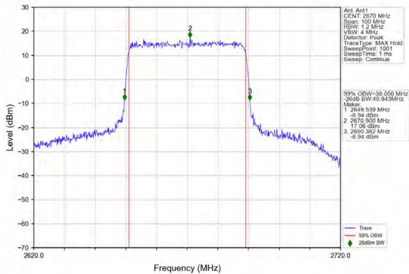
n41_30kHz_SISO_NTNV_40MHz_CP-OFDM_QPSK_2670MHz_Outer_Full
