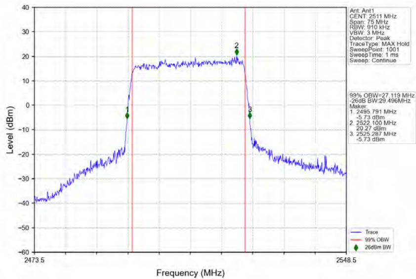
n41_30kHz_SISO_NTNV_30MHz_DFT-s-OFDM_QPSK_2511MHz_Outer_Full
