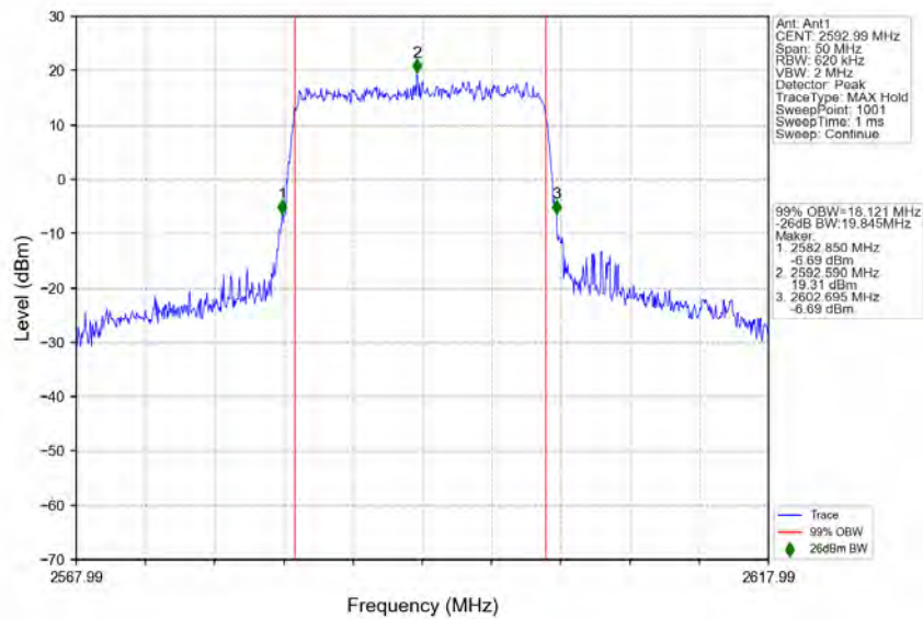
n41_30kHz_SISO_NTNV_20MHz_DFT-s-OFDM_16_QAM_2592.99MHz_Outer_Full
