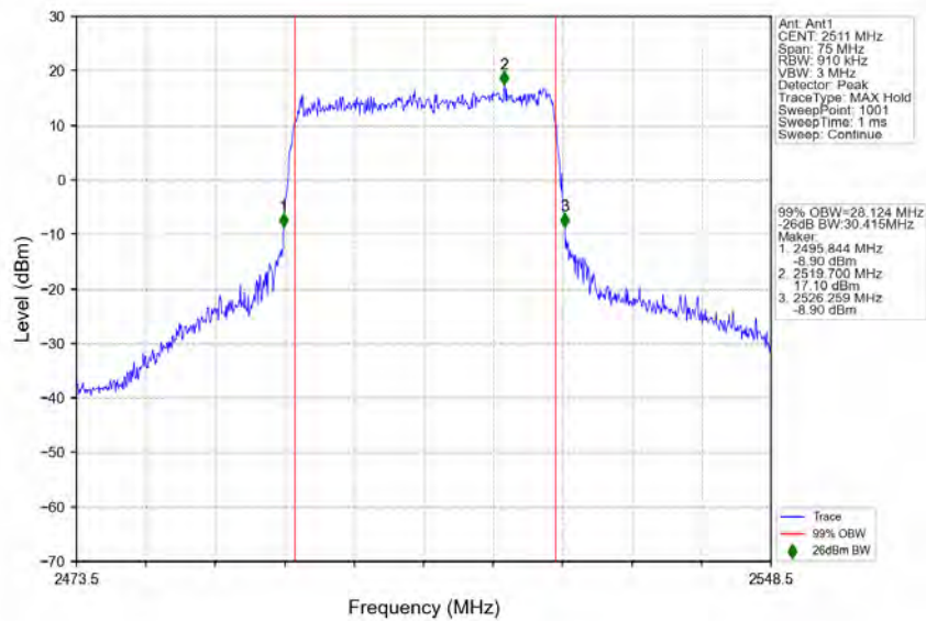
n41_30kHz_SISO_NTNV_30MHz_CP-OFDM_64_QAM_2511MHz_Outer_Full
