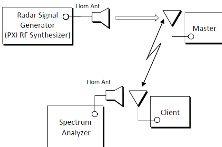
Figure 8-1. Test Setup
