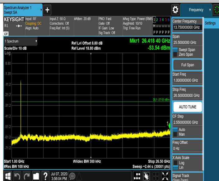
11N40SISO_Ant1_2422_0~Reference
