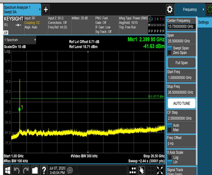
11N20SISO_Ant1_2437_0~Reference
