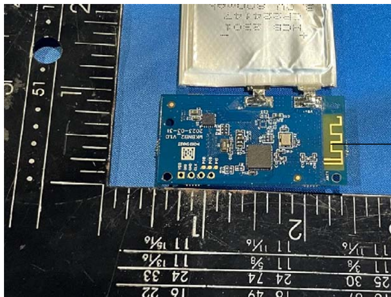
2402-2480MHz BT Antenna
