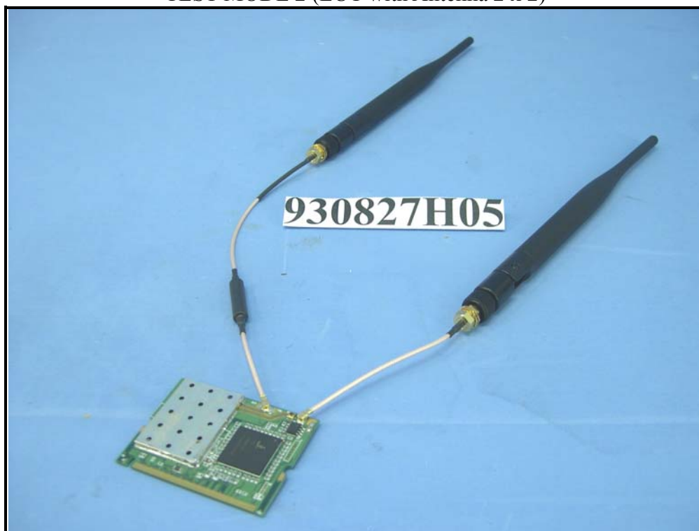
TEST MODE 2 (EUT with Antenna 2 x 2)
