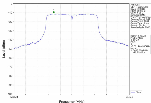
(802.11ac20) PSD plot on channel 165
