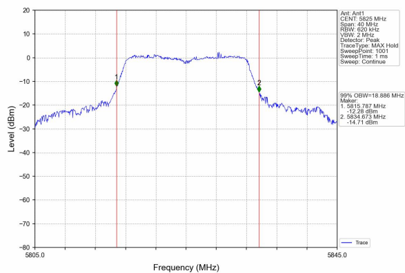
(802.11a) channel 165
