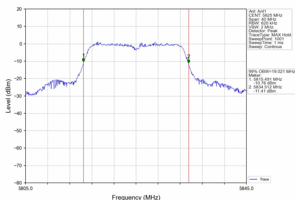
(802.11n20) channel 165
