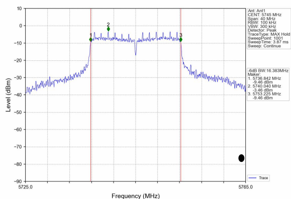
(802.11a) -6dB Bandwidth plot on channel 149
