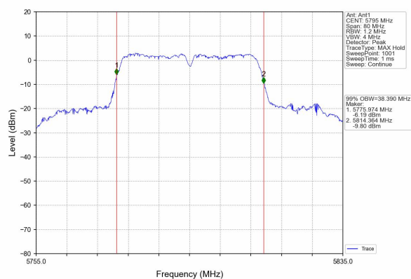
(802.11 n40) channel 159
