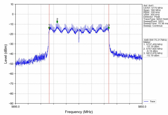
(802.11 ac80) -6dB Bandwidth plot on channel 155
