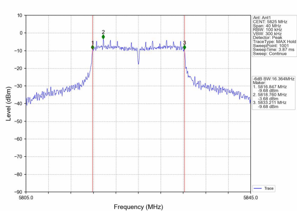
(802.11a) -6dB Bandwidth plot on channel 165
