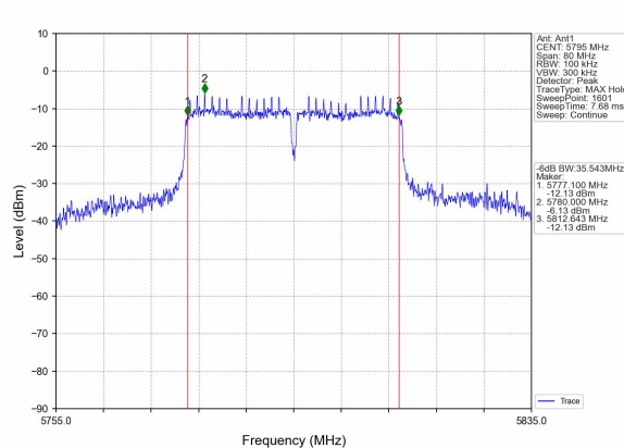
(802.11 n40) -6dB Bandwidth plot on channel 159
