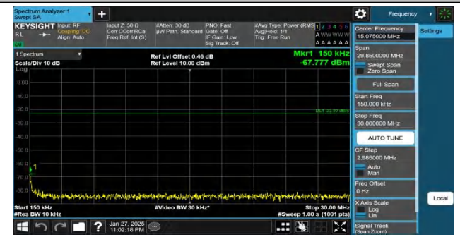
Band26(824-849)-15MHz-QPSK-26915-1RB#0-0.15~30-PASS
