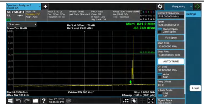
Band26(824-849)-5MHz-QPSK-27015-1RB#24-30~1000-PASS
