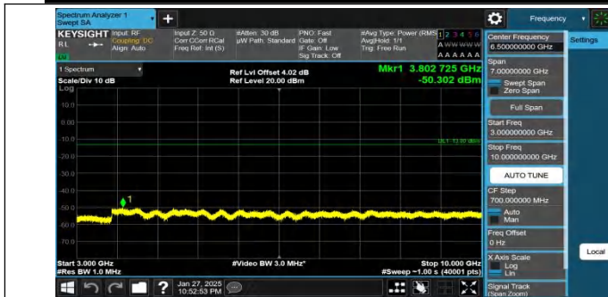
Band26(824-849)-10MHz-QPSK-26915-1RB#0-3000~10000-PAS
