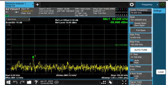
Band26(824-849)-5MHz-QPSK-27015-1RB#24-0.009~0.15-PASS
