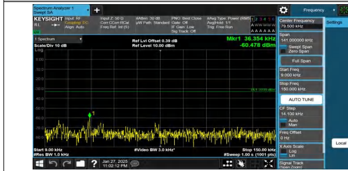
Band26(824-849)-15MHz-QPSK-26915-1RB#0-0.009~0.15-PASS
