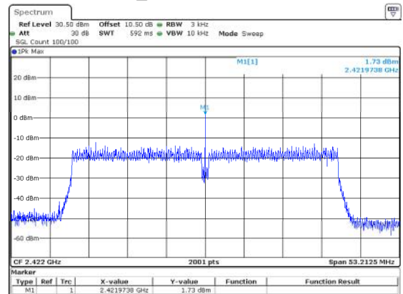
802.11n40_2422MHz 1.73dBm/3kHz
