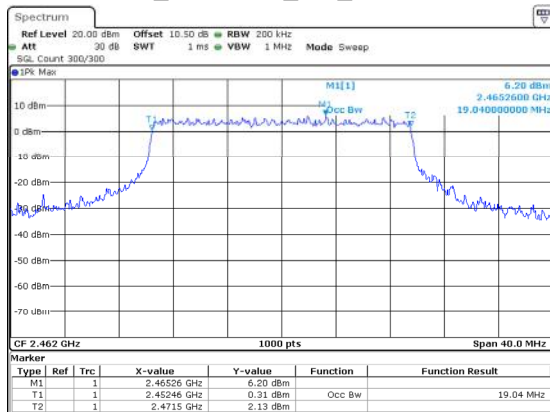
802.11ax20_2462MHz_RU_Full 19.040MHz
