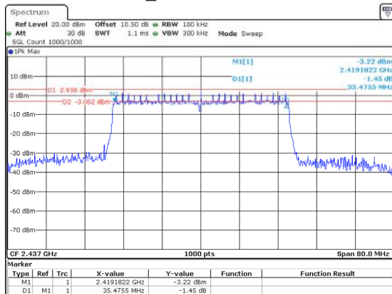
802.11n40_2437MHz 35.475MHz
