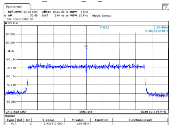
802.11ax40_2452MHz_RU_Full 1.89dBm/3kHz
