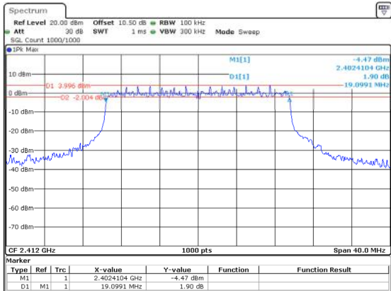
802.11ax20_2412MHz_RU_Full 19.099MHz
