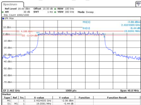
802.11ax20_2462MHz_RU_Full 19.059MHz
