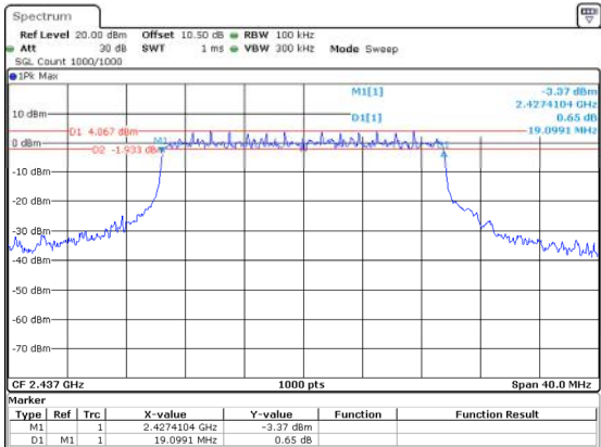
802.11ax20_2437MHz_RU_Full 19.099MHz
