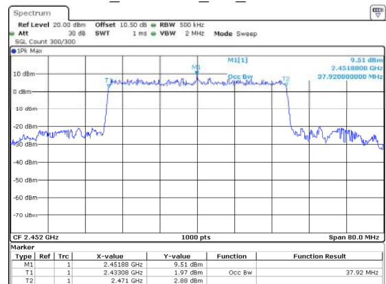
802.11ax40_2452MHz_RU_Full 37.920MHz
