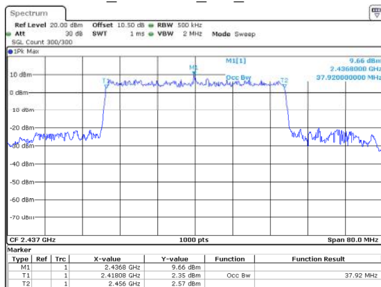
802.11ax40_2437MHz_RU_Full 37.920MHz
