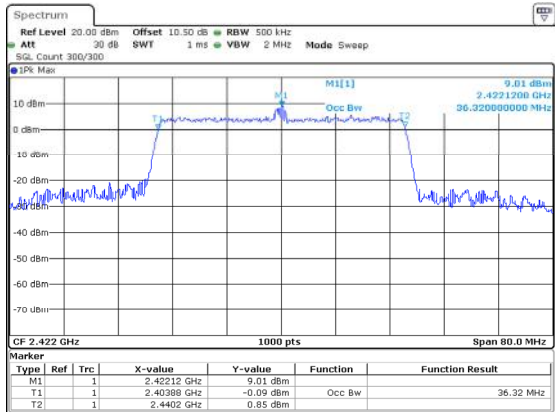
802.11n40_2422MHz 36.320MHz
