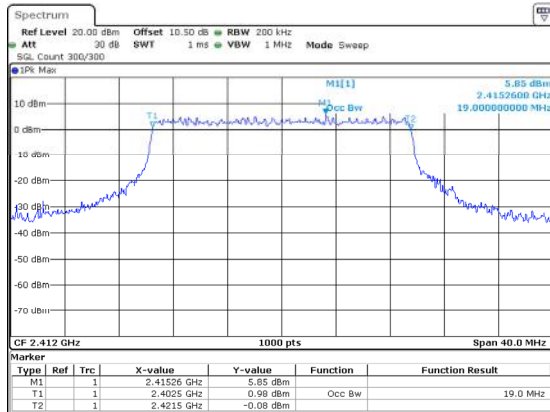
802.11ax20_2412MHz_RU_Full 19MHz
