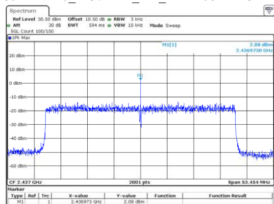
802.11ax40_2437MHz_RU_Full 2.08dBm/3kHz
