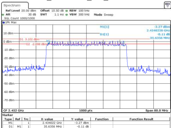
802.11ax40_2452MHz_RU_Full 35.636MHz
