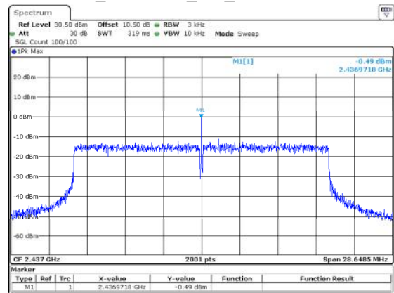
802.11ax20_2437MHz_RU_Full -0.49dBm/3kHz
