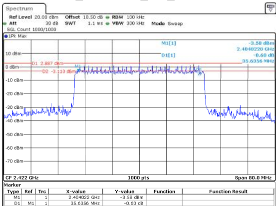
802.11ax40_2422MHz_RU_Full 35.636MHz
