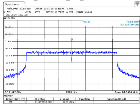
802.11ax20_2412MHz_RU_Full -0.60dBm/3kHz
