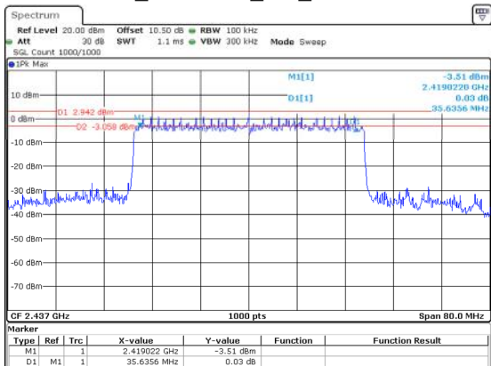
802.11ax40_2437MHz_RU_Full 35.636MHz
