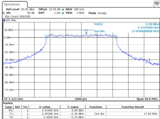
802.11n20_2412MHz 17.840MHz
