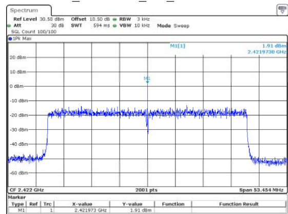
802.11ax40_2422MHz_RU_Full 1.91dBm/3kHz
