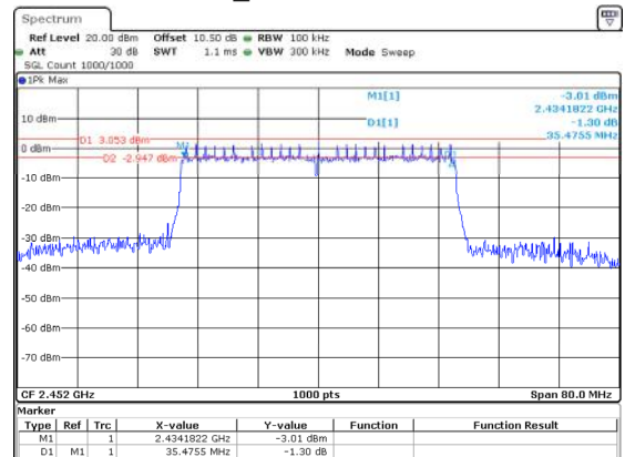
802.11n40_2452MHz 35.475MHz
