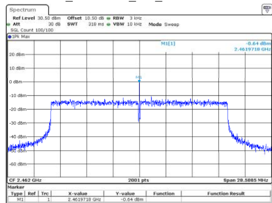
802.11ax20_2462MHz_RU_Full -0.64dBm/3kHz
