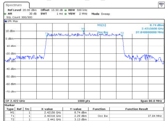
802.11ax40_2422MHz_RU_Full 37.840MHz
