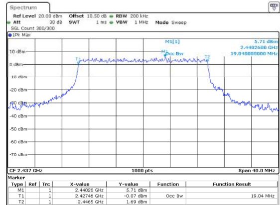
802.11ax20_2437MHz_RU_Full 19.040MHz
