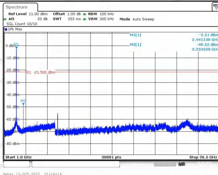
20M_Ant2_2440_0~Reference
