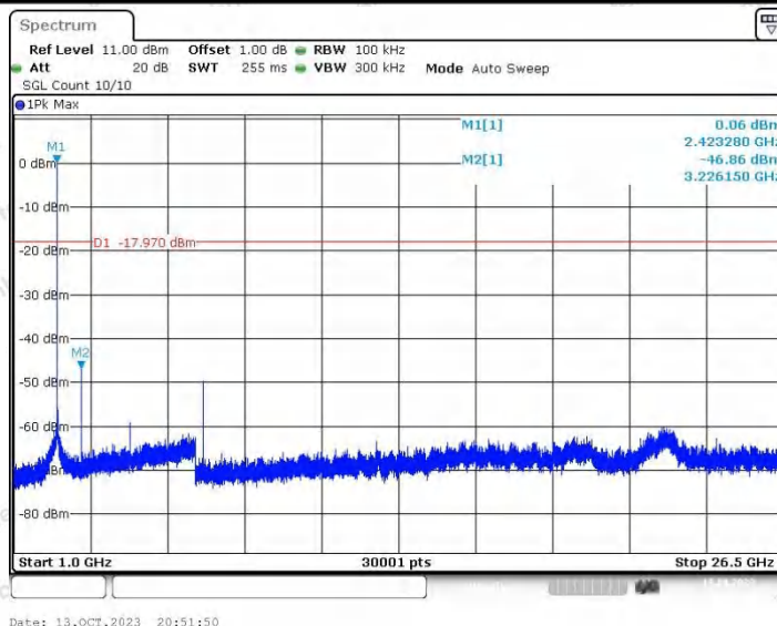
10M_Ant2_2420_0~Reference
