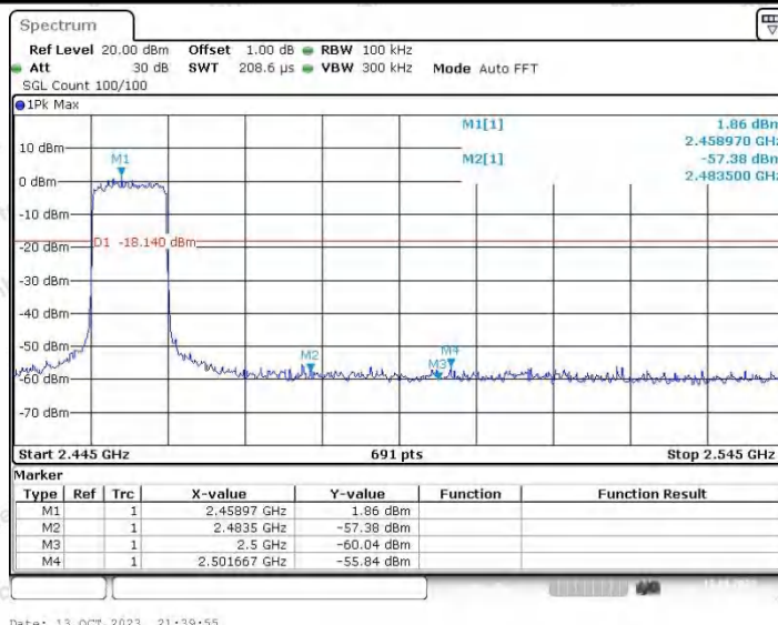
10M_Ant2_High_2460
