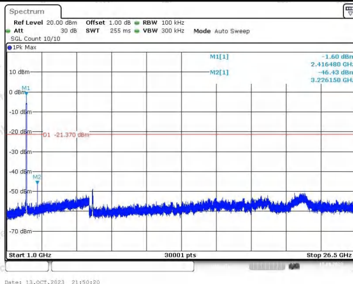
40M_Ant2_2420_0~Reference
