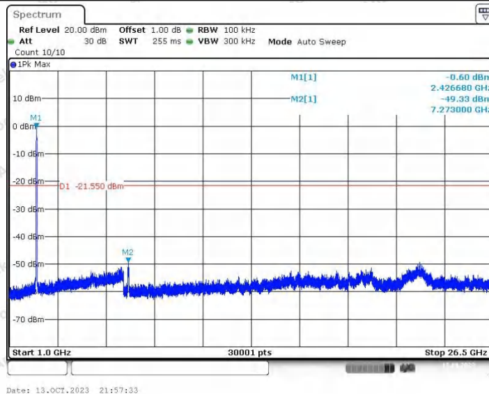
40M_Ant1_2440_0~Reference
