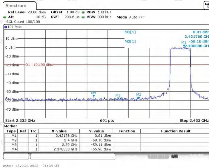
10M_Ant2_Low_2420
