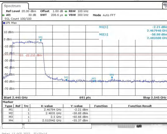
20M_Ant2_High_2460
