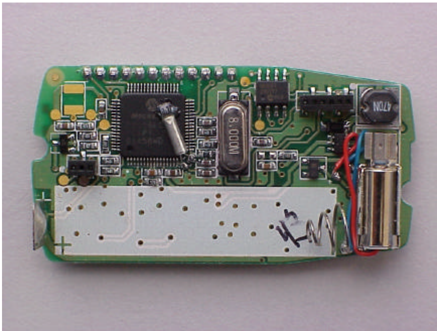
Bottom view of DB19 PCB.
