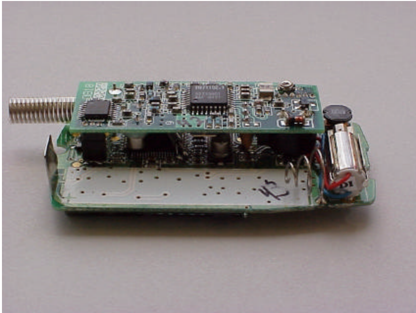
DB18 and DB19 PCB assemblies in top of the case assembly
