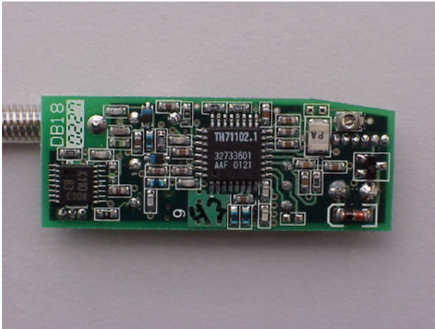
BOTTOM VIEW OF DB18
