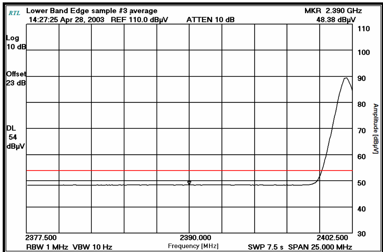
PLOT 3-5: LOWER BAND EDGE: AVERAGE MEASUREMENT QL-220
