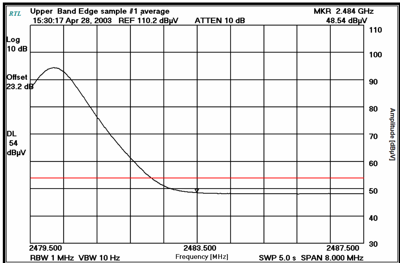
PLOT 3-13: UPPER BAND EDGE: AVERAGE MEASUREMENT CAMEO 3
