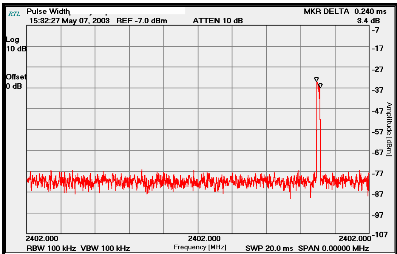
PLOT 8-2: TIME OF OCCUPANCY (DWEELL TIME)
