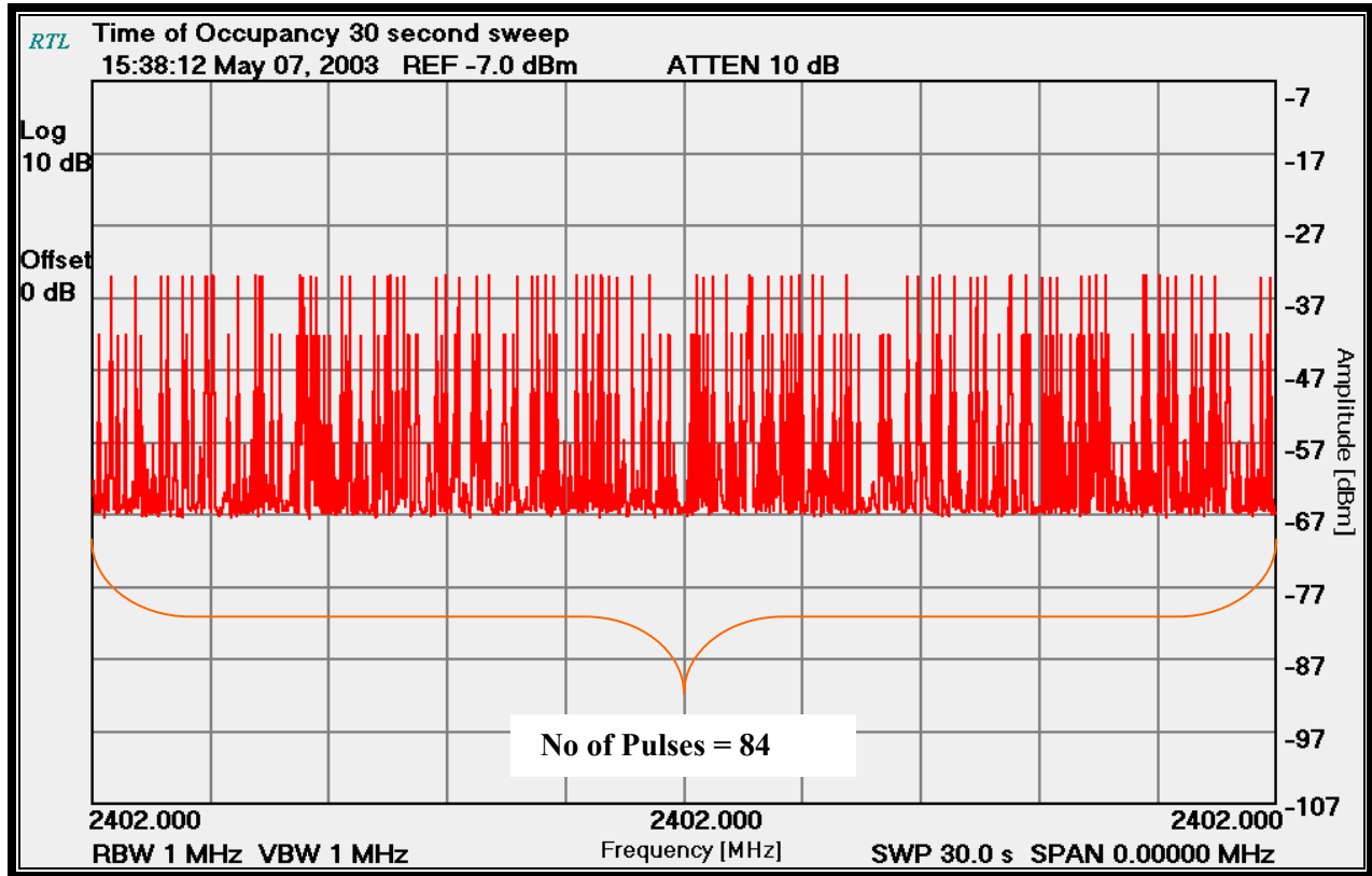
PLOT 8-3: TIME OF OCCUPANCY (DWELL TIME 30 SECOND SWEEP)
