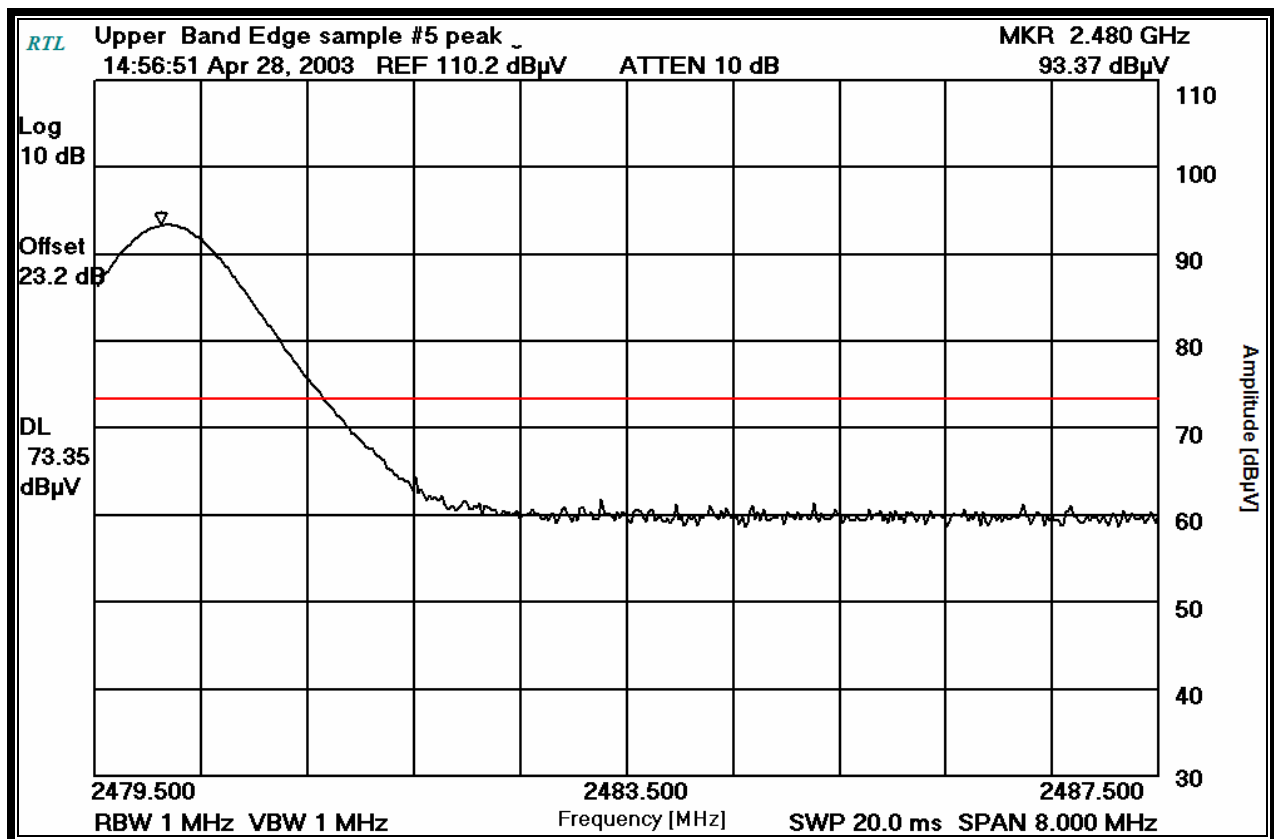
PLOT 3-22: UPPER BAND EDGE: PEAK MEASUREMENT QL-320
