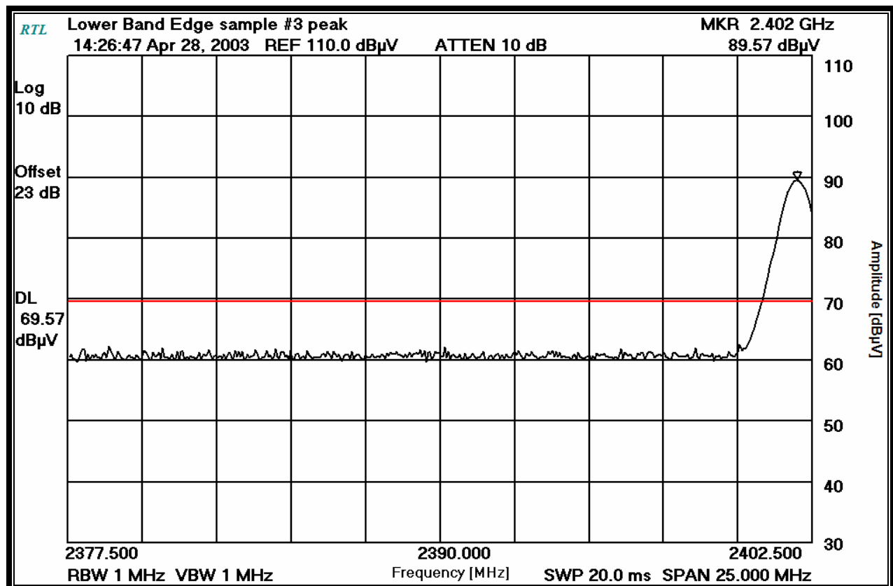
PLOT 3-6: LOWER BAND EDGE: PEAK MEASUREMENT QL-220
