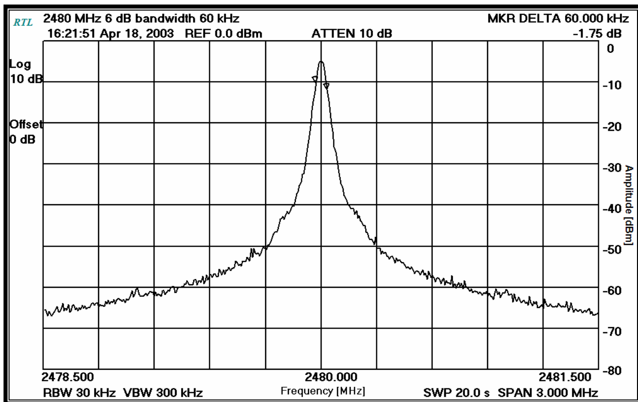
PLOT 9-3: MODULATED BANDWIDTH CHANNEL 80
