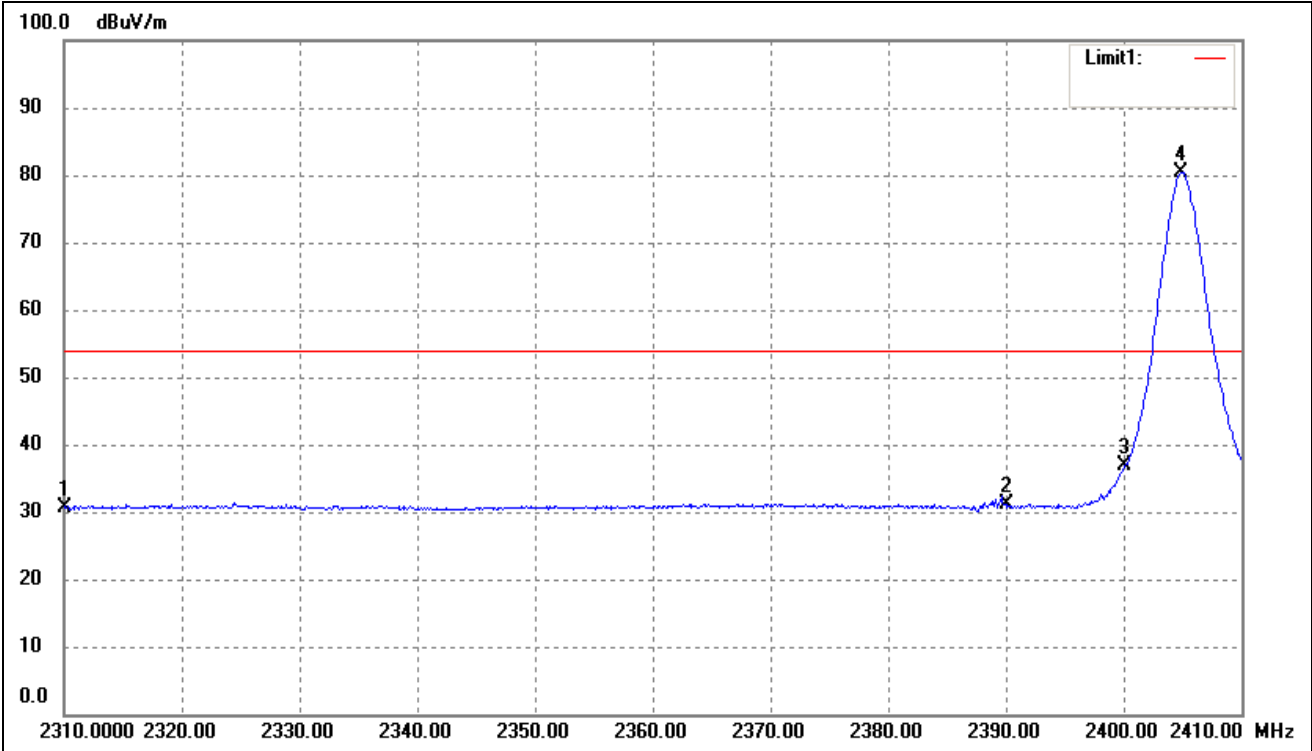
Lowest Bandedge
