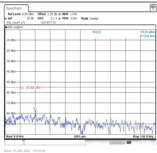
Band41_15MHz_16QAM_40315_1RB#0_0.009~0.15
