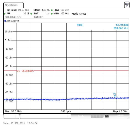
Band41_15MHz_16QAM_40315_1RB#0_30~1000
