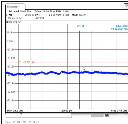
Band41_15MHz_QPSK_40315_1RB#0_20000~27000
