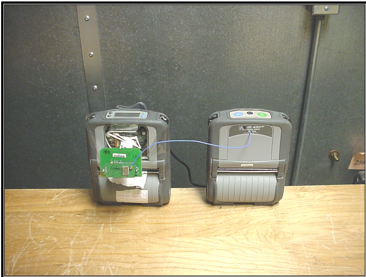
PHOTOGRAPH 18: CONDUCTED EMISSIONS FRONT VIEW
