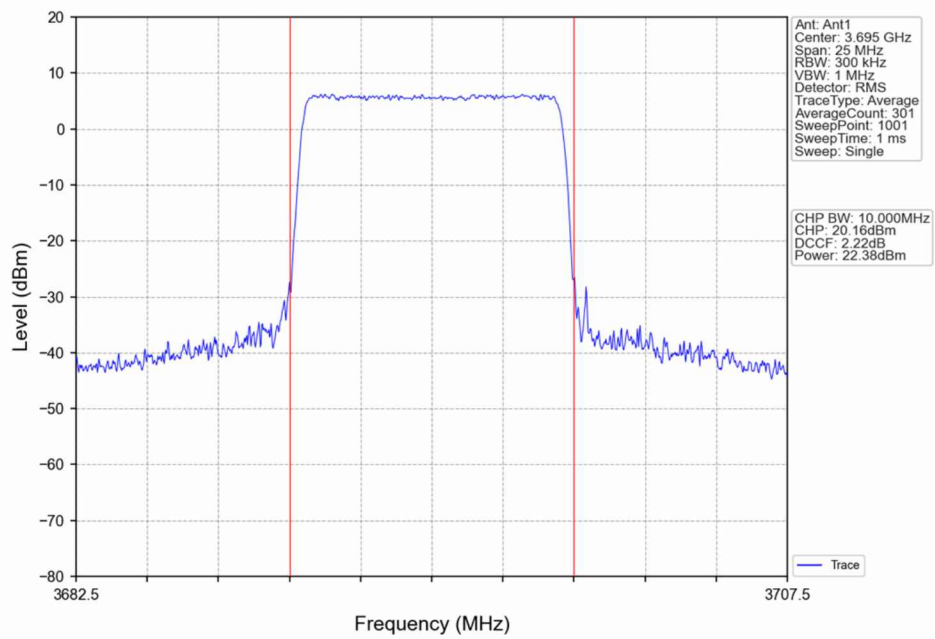
Band48_10MHz_16QAM_HCH_3695MHz_RB_50_0_NTNV
