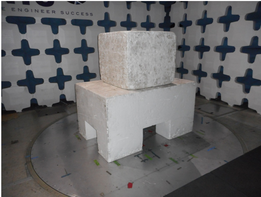
TX spurious 1 GHz - Front
