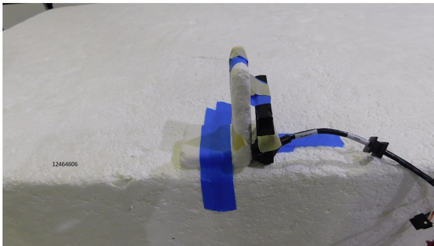
RADIATED EMISSIONS – Y ORIENTATION
