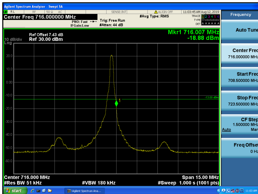
LTE Band 12, 17 / 5MHz / QPSK - RB Size/Offset (15/0)
