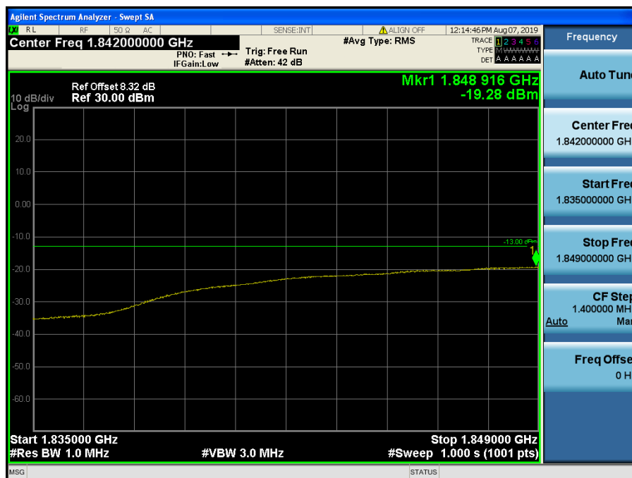
LTE Band 2 / 15MHz / 16QAM - RB Size/Offset (75/0)
