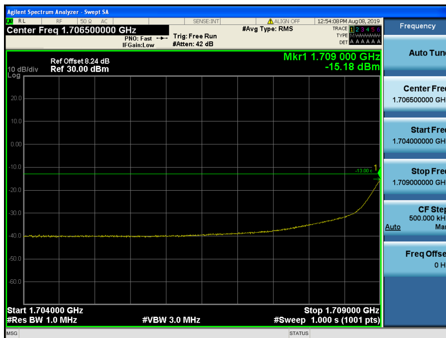
LTE Band 4 / 1.4MHz / 16QAM - RB Size/Offset (3/2)
