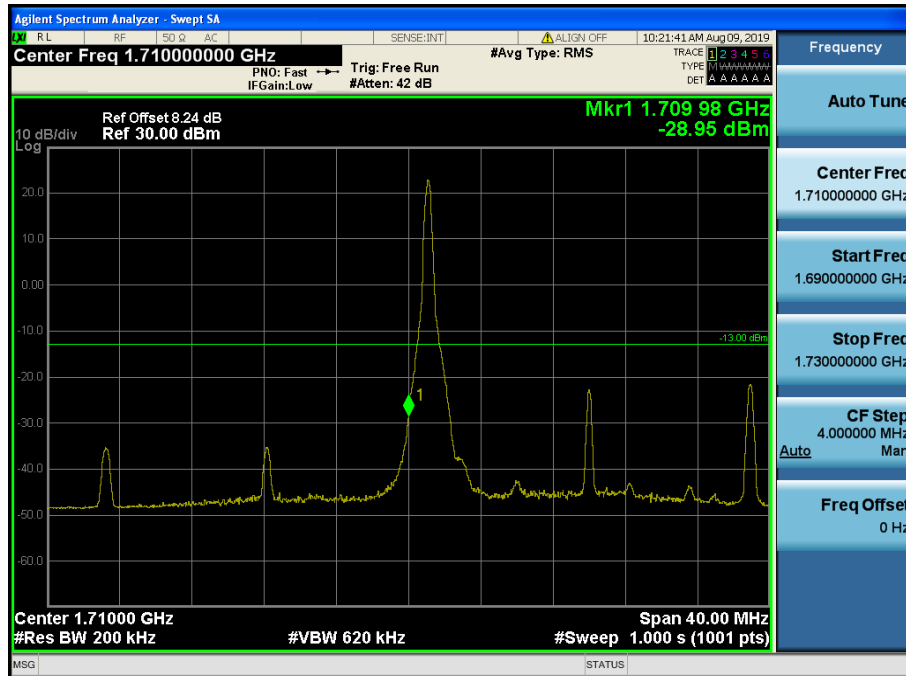
LTE Band 4 / 20MHz / 16QAM - RB Size/Offset (1/0)
