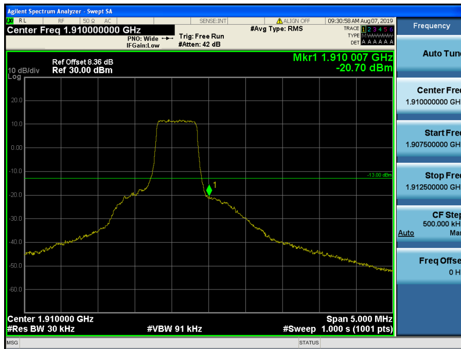
LTE Band 2 / 1.4MHz / 16QAM - RB Size/Offset (3/3)
