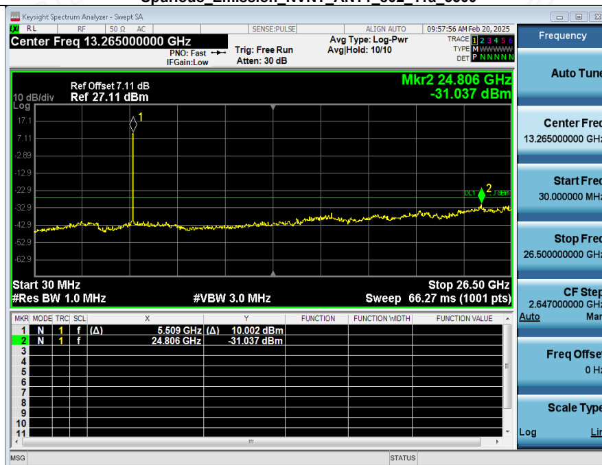
Spurious Emission_NVNT_ANT2_802_11a_5500
