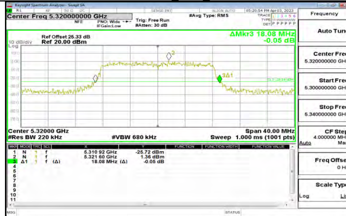
11A-CDD Ant9 5320
