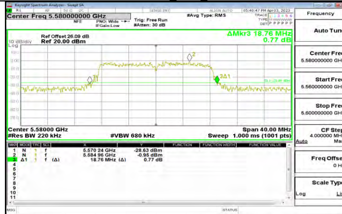
11A-CDD Ant10 5580
