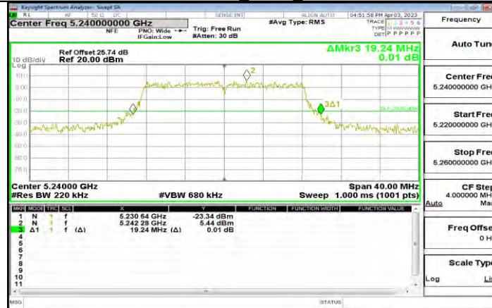
11A-CDD Ant15 5240
