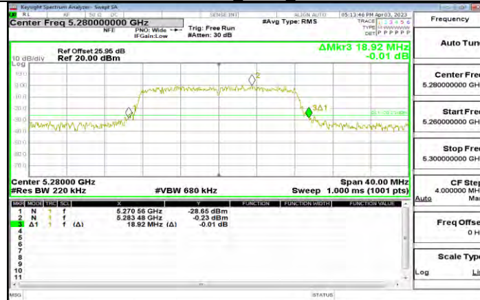
11A-CDD Ant15 5280
