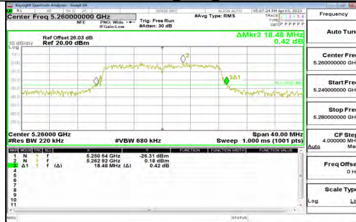
11A-CDD Ant16 5260
