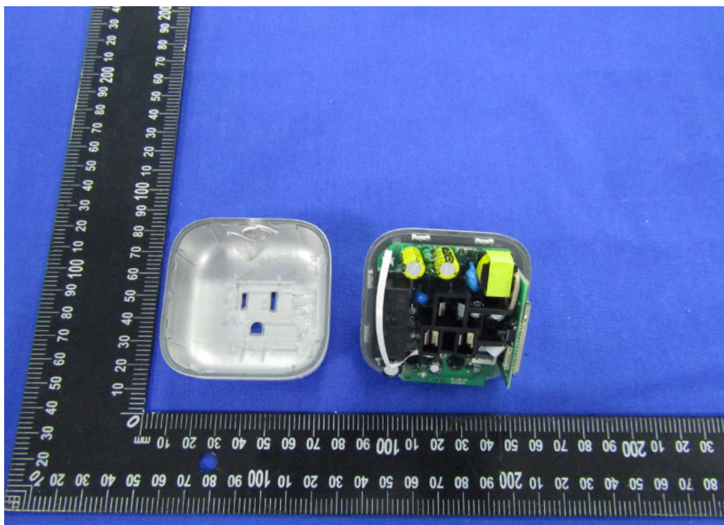
EUT –Uncovered View
