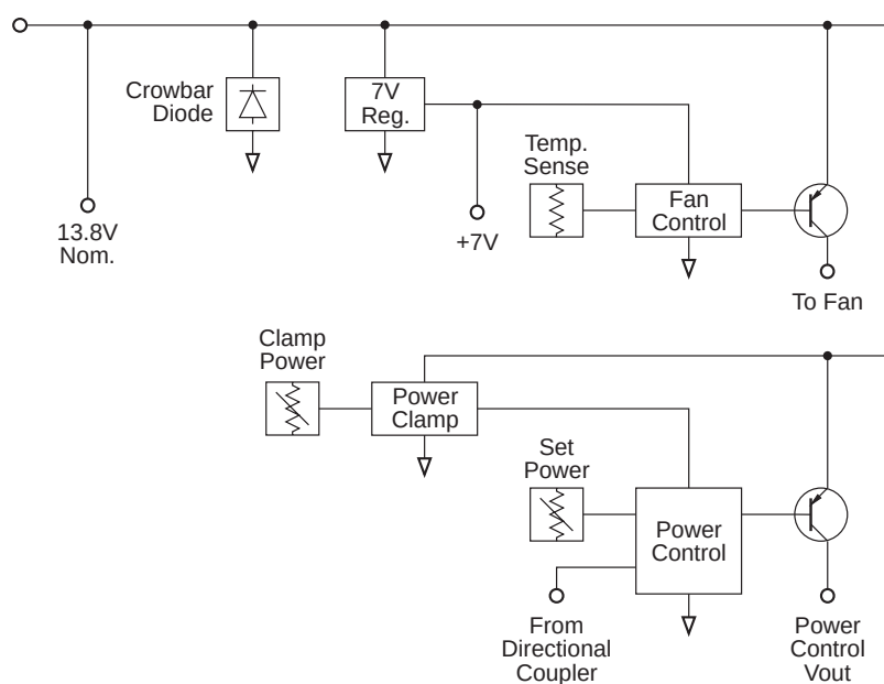
Figure 2.11 T858/859 Power Supply & Regulator Circuitry Block Diagram
